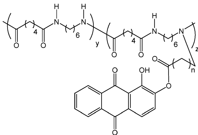
Compound 4: alizarin-modified Nylon 6,6
