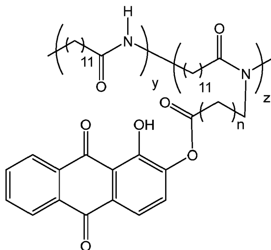
Compound 3: alizarin-modified Nylon 12
