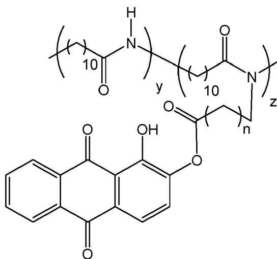
Compound 2: alizarin-modified Nylon 11
