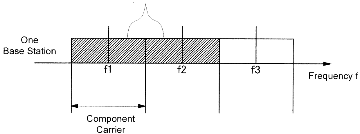
Component Carrier used for Band Aggregation in the above Diagram
