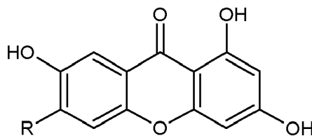
Ia: R = 1,5-anhydro-D-glucitol
