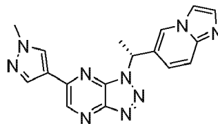
Compound 271
