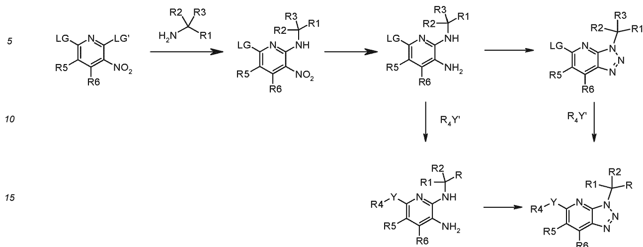
Scheme II
