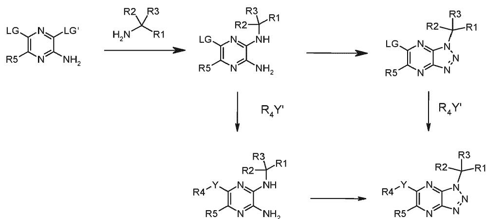
Scheme I
