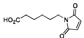
6-maleimido hexanoic acid Commercially available
