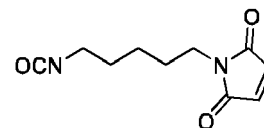
colorless oil Compound 2' (isocyanate) MW: 208.22
