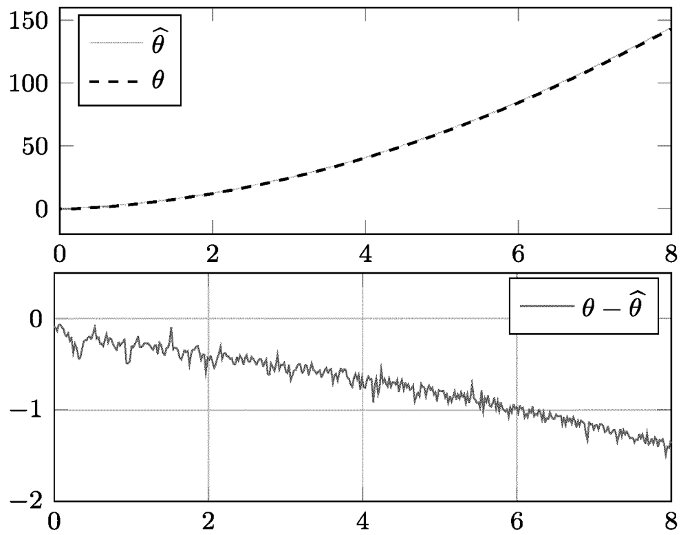
Fig. 20: Reconstruction of \theta in rad (experiment).
