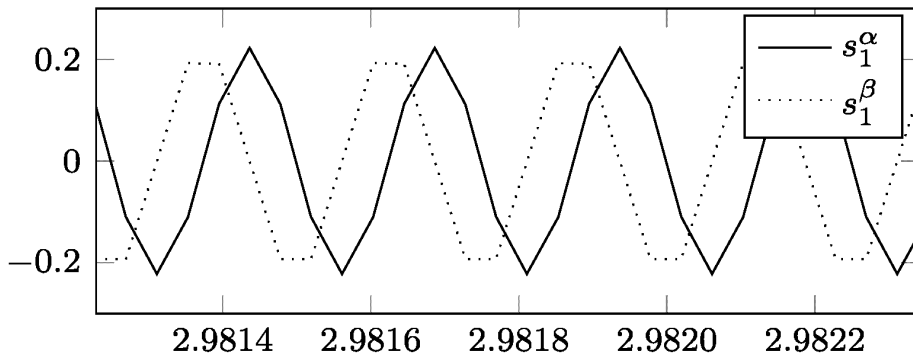
Fig. 14: s_1^{\alpha\beta} for interleaved PWM (simulation data).
