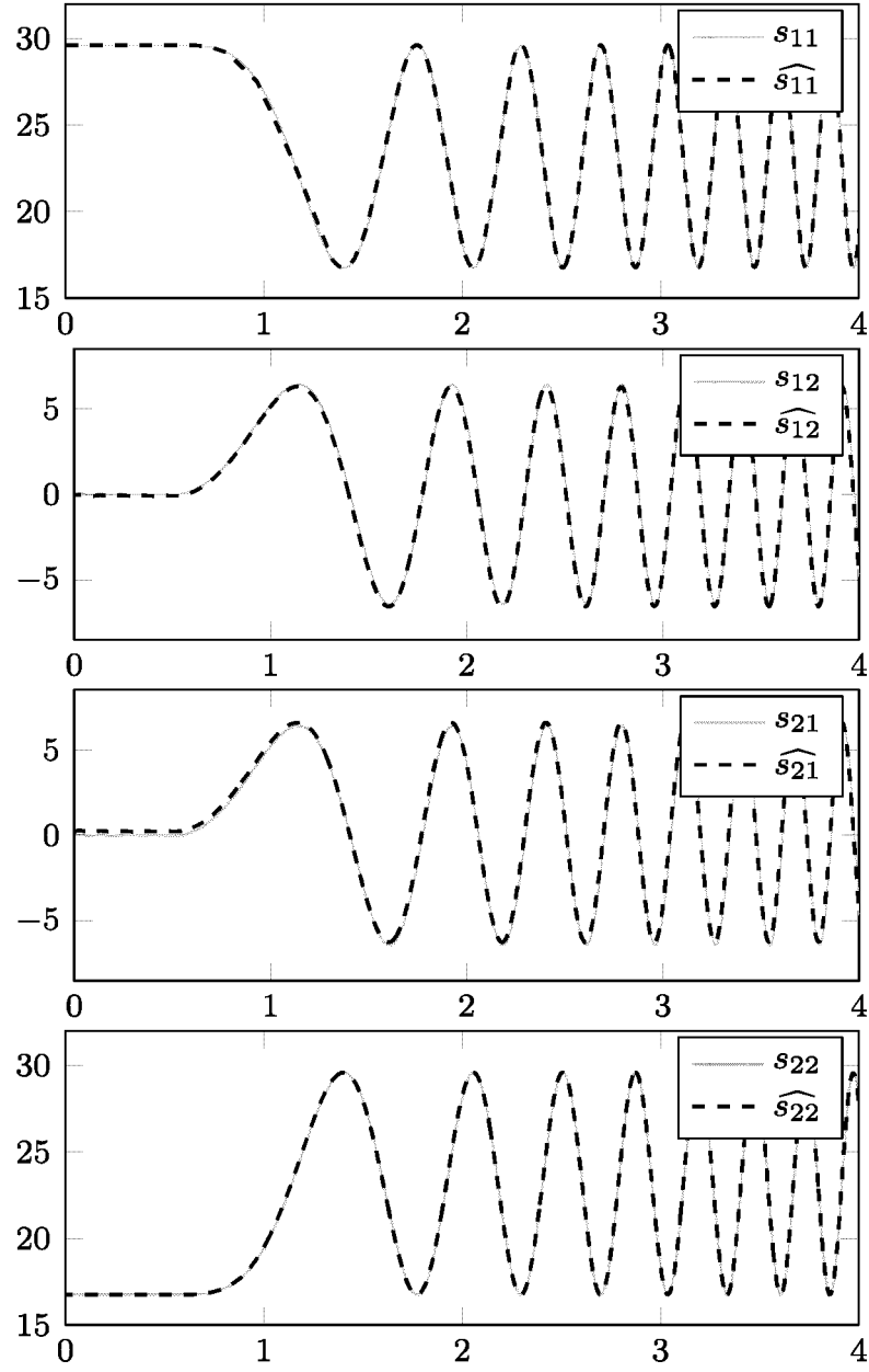
Fig. 21: Reconstruction of saliency matrix S(\theta) (simulation).
