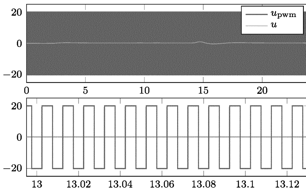
Fig. 6: Control input u and its modulation u_{\text{pwm}} ; full view (top), zoom (bottom).
