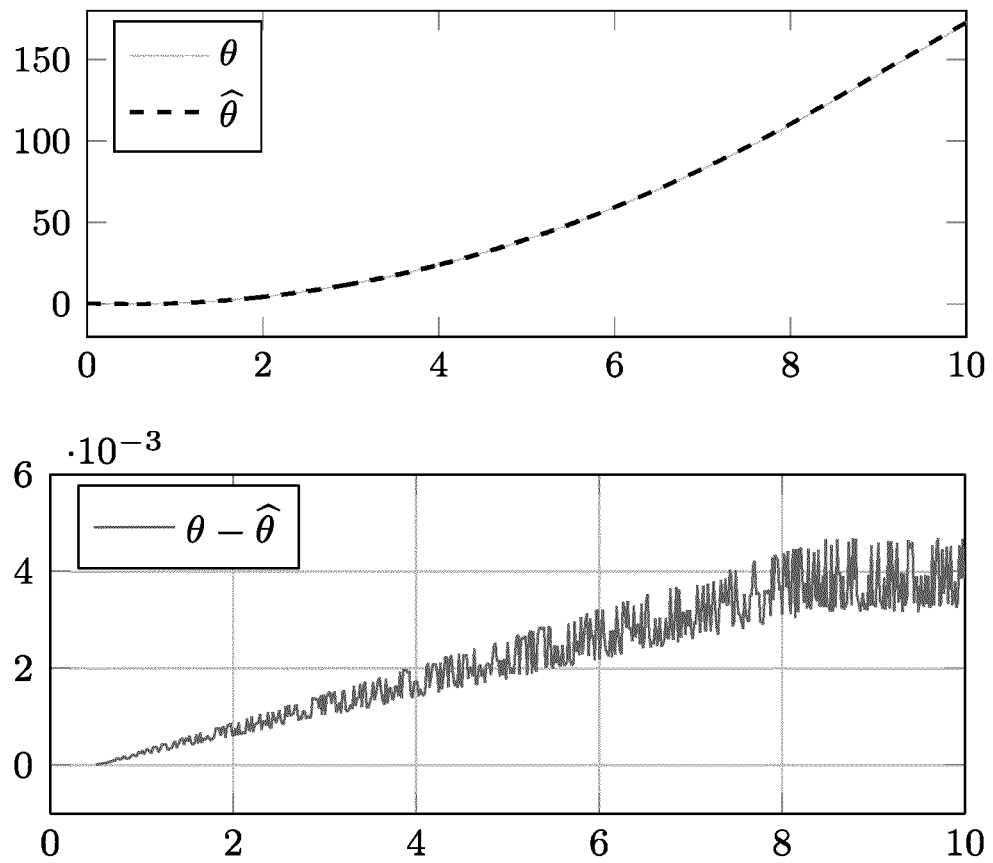
Fig. 16: Reconstruction of \theta in rad (simulation).
