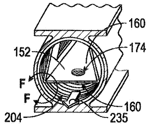
FIG. 6B (Section B-B)
