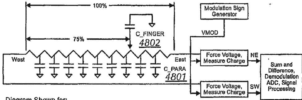
Diagram Shown for: "Measure X" On "Measure XY" On "Measure Y" Off C_PARA is parasitic capacitance distributed across touch panel. C_FINGER is signal capacitance associated with a touch on the touch panel.
