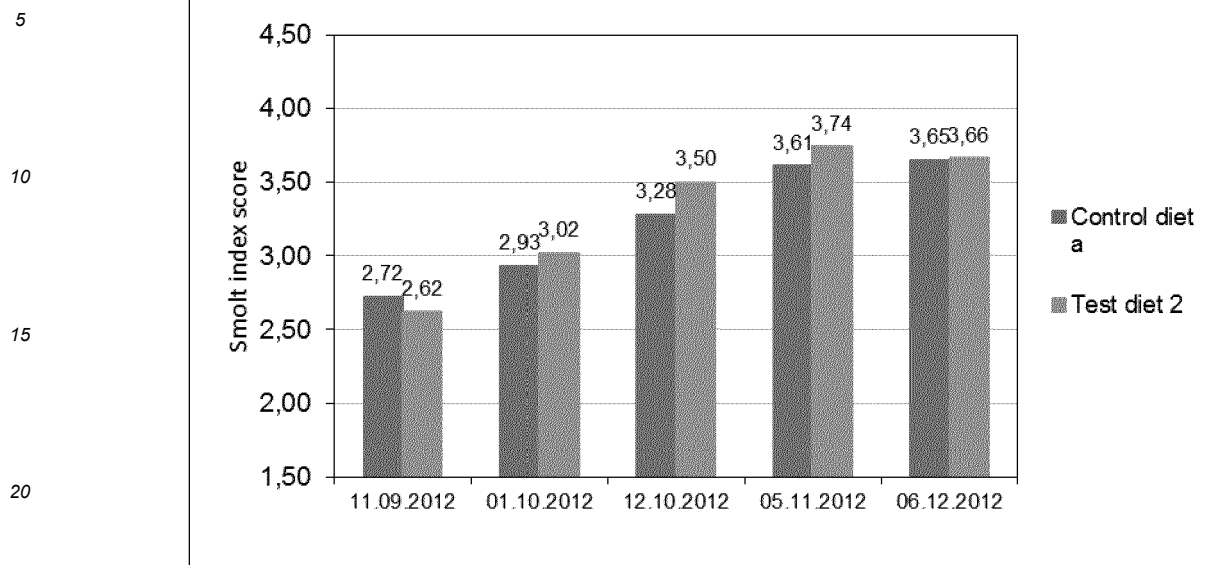
Diagram 12: Development of the average smolt index by continuously light, in fish that
