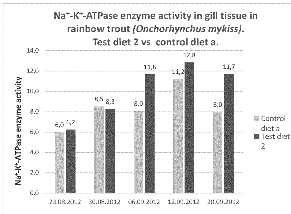
Diagram 7: Development of the average Na + -K + -ATPase enzyme activity in gill tissue after the winter signal (12 hours light/12 hours dark), in Rainbow trout received test diet 2 and control diet a. (n = 25/sampling in each group). The trial is from cages in freshwater lake (4 test cages and 4 control cages), Chile. Removal by grading, of the smallest fish before delivery, made between 12. and 20. of September 2012.
