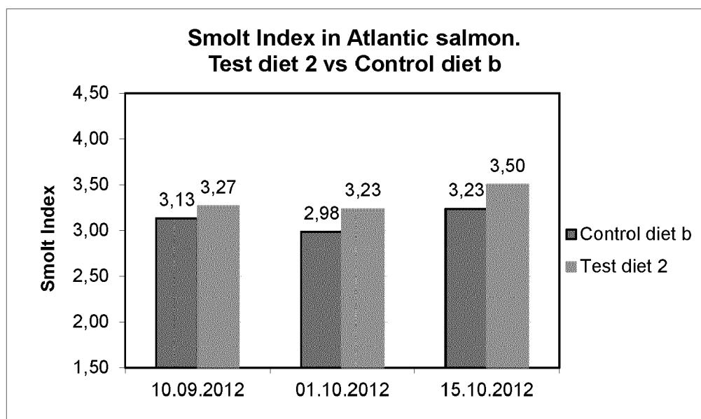
Diagram 18: Development of the average smolt index of Atlantic salmon under natural light conditions, when feeding of Atlantic salmon with test diet 2, vs control diet b. ( n = 20 /sampling point in each group).
