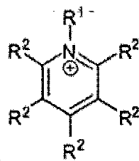
Formula XVIII,
