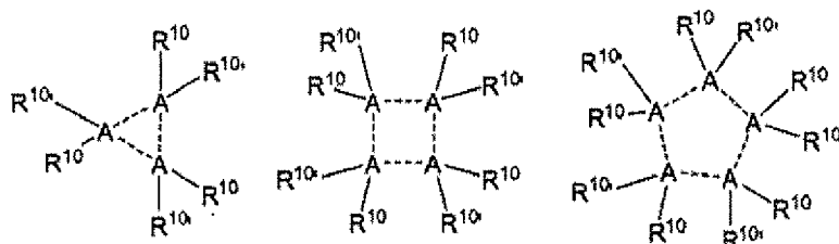
Formula V
