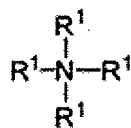
Formula XXI
