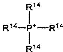
Formula XII
