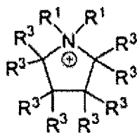
Formula (II),
