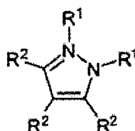
Formula (IV)
