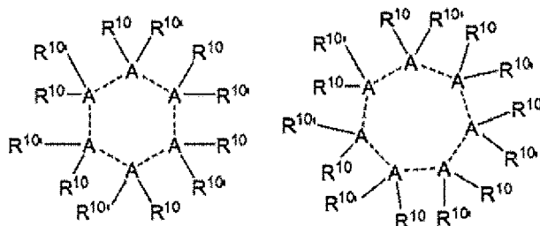
Formula VIII
