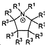
Formula XVII,
