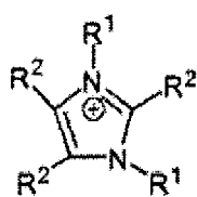
Formula XVI,
