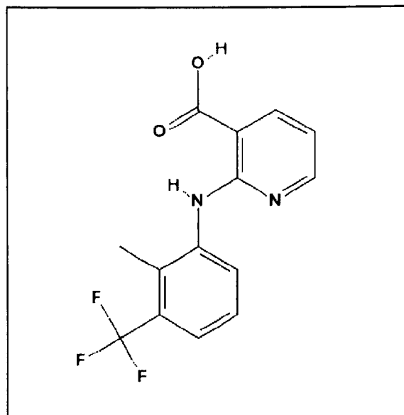
flunixin
