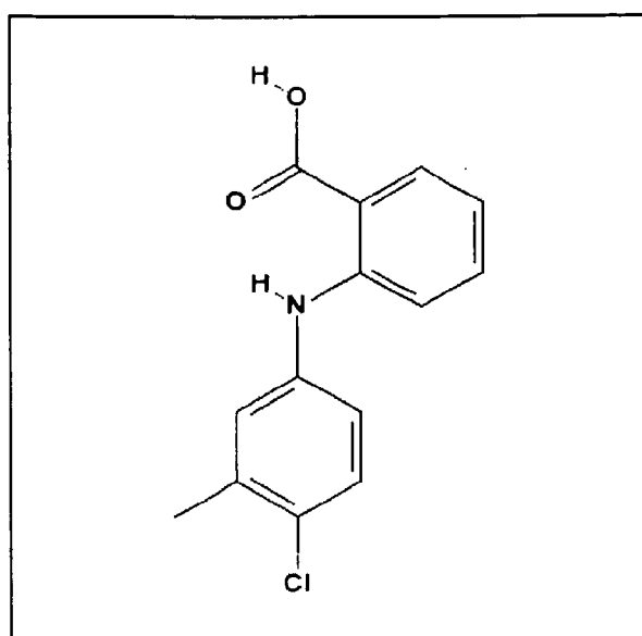
Tolfenamic acid
