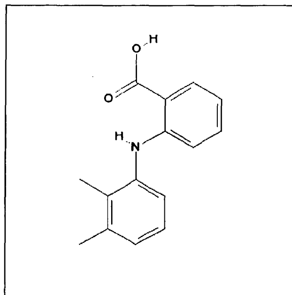
Mefenamic acid
