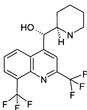
(R,R)-mefloquine
