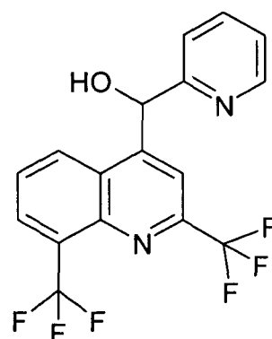
(2,8-Bis-trifluoromethyl-quinolin-4-yl)-pyridin-2-yl-methanol
