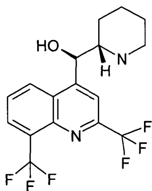
(S,S)-mefloquine
