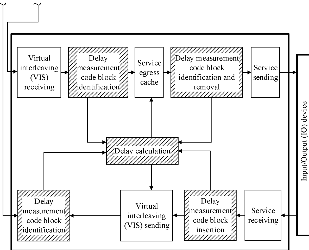
Third switch device (VIS 3)-Edge device
