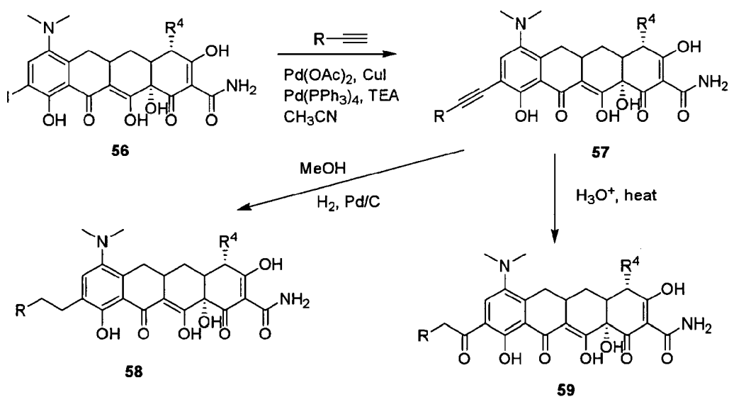
Scheme 26
