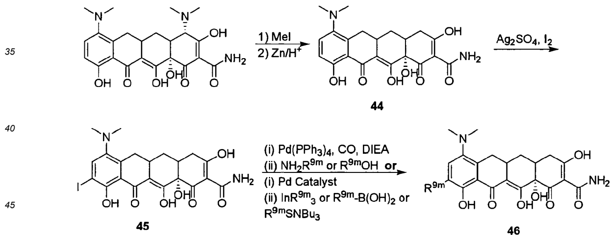
Scheme 21
