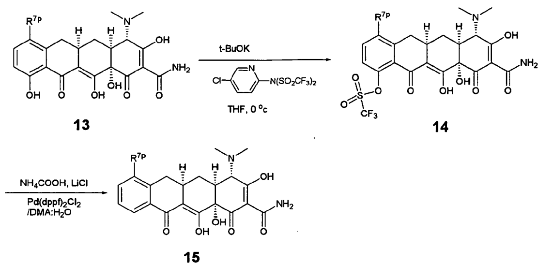
Scheme 5
