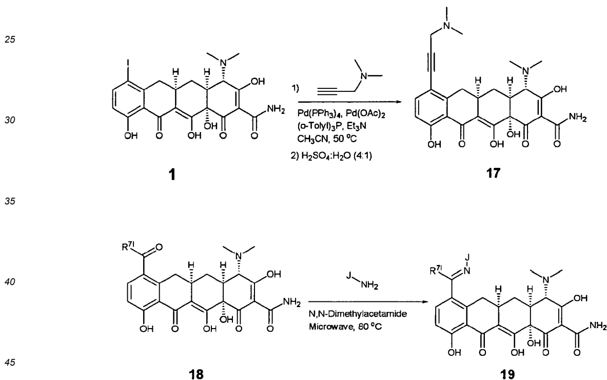
Scheme 7
