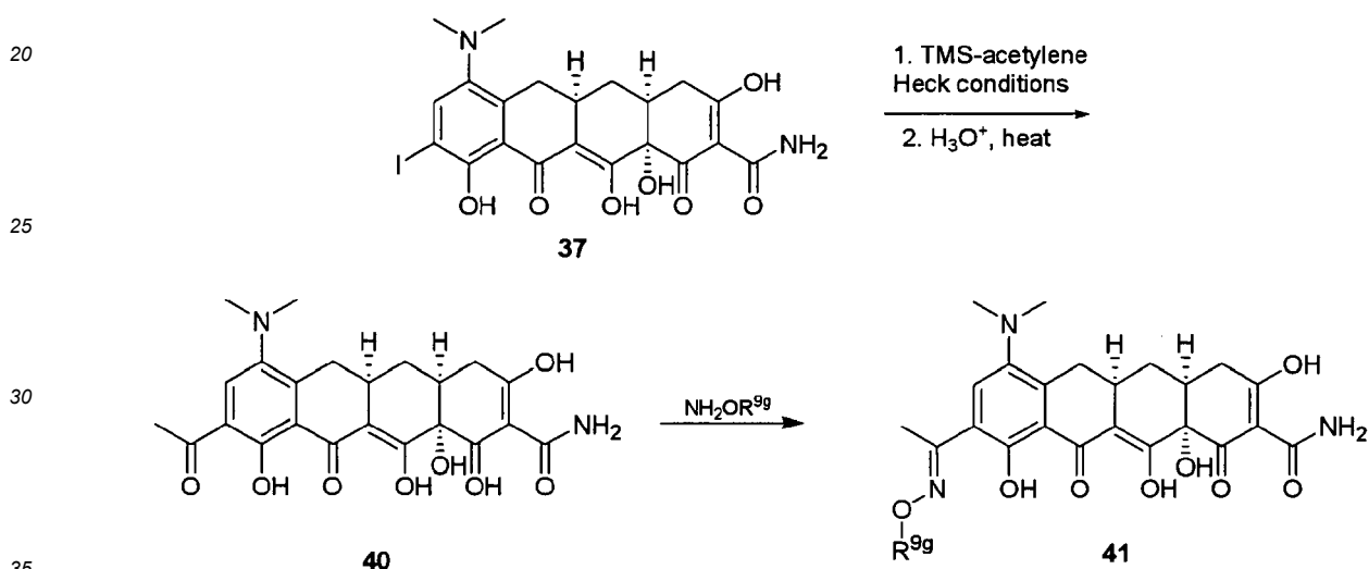
Scheme 19
