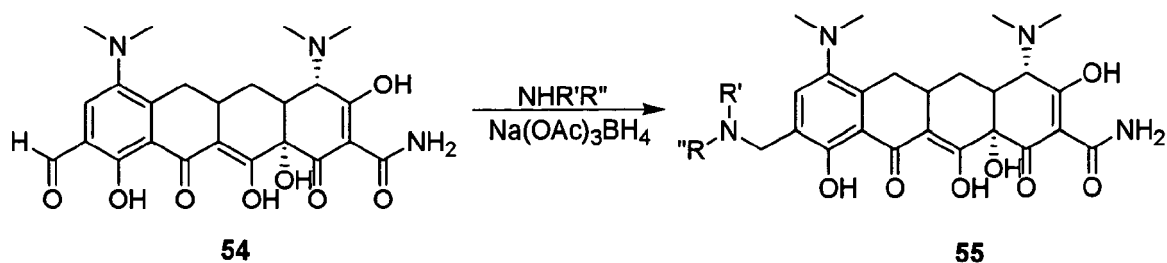
Scheme 25
