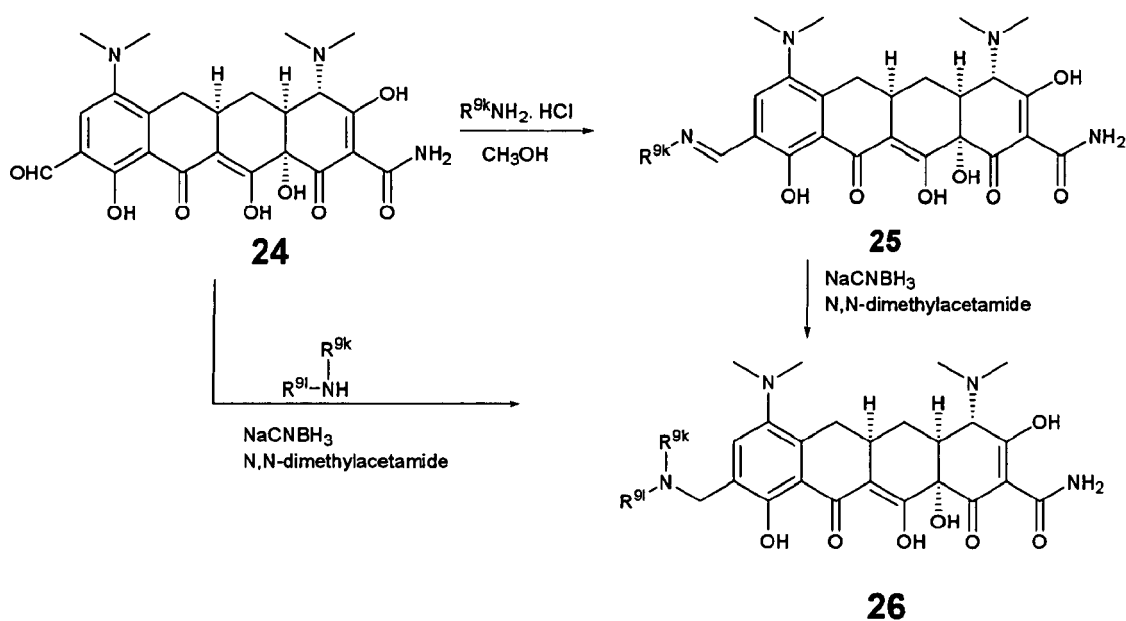
Scheme 11
