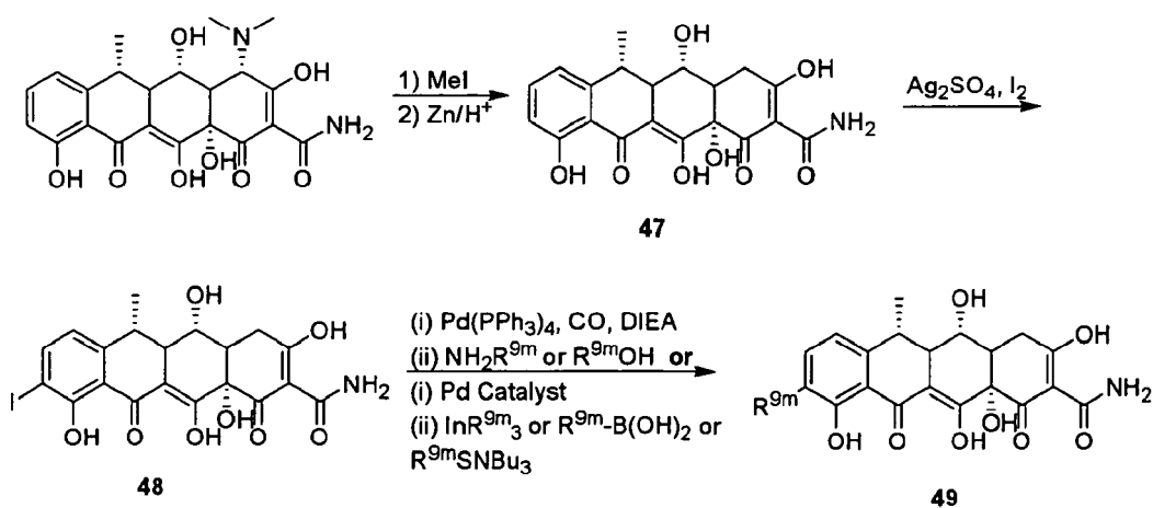
Scheme 22
