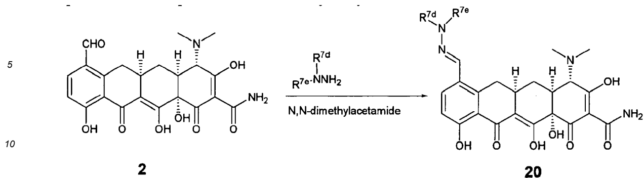
Scheme 8
