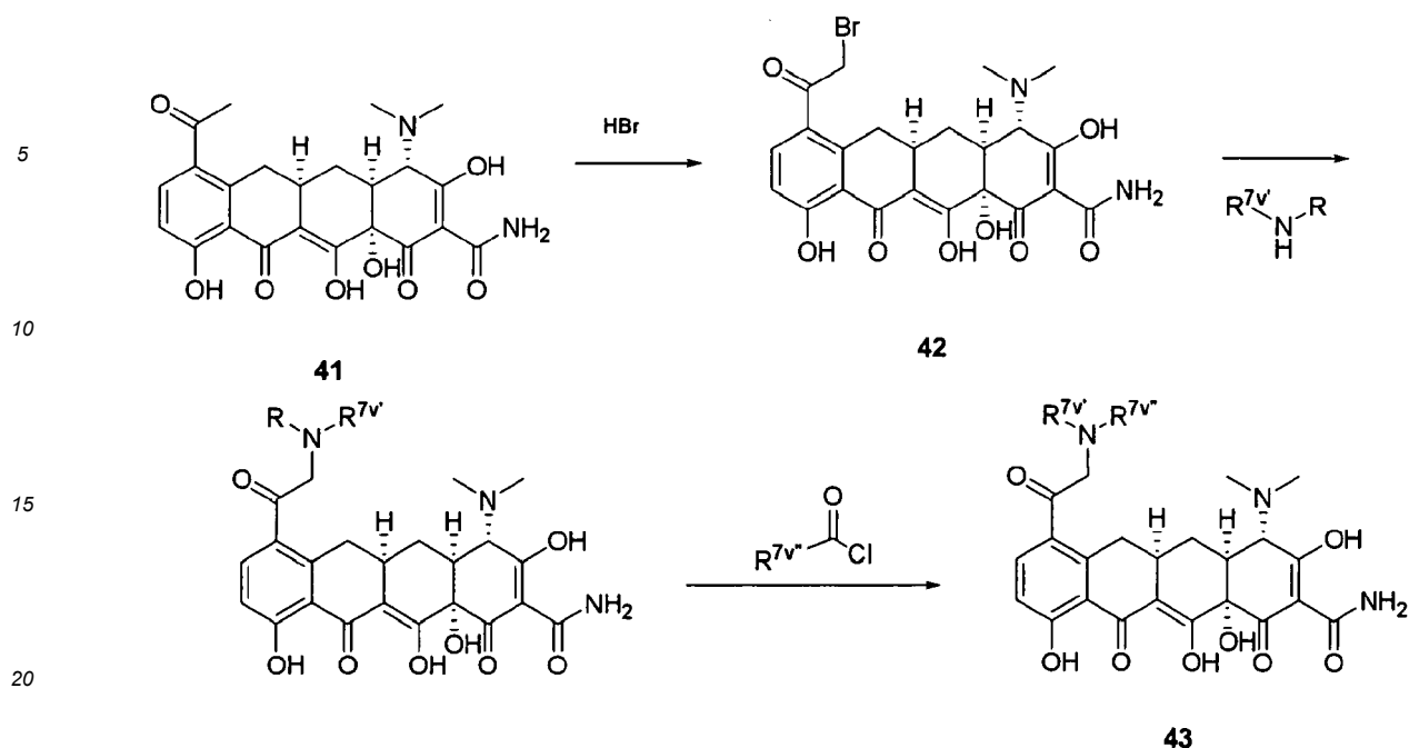
Scheme 20
