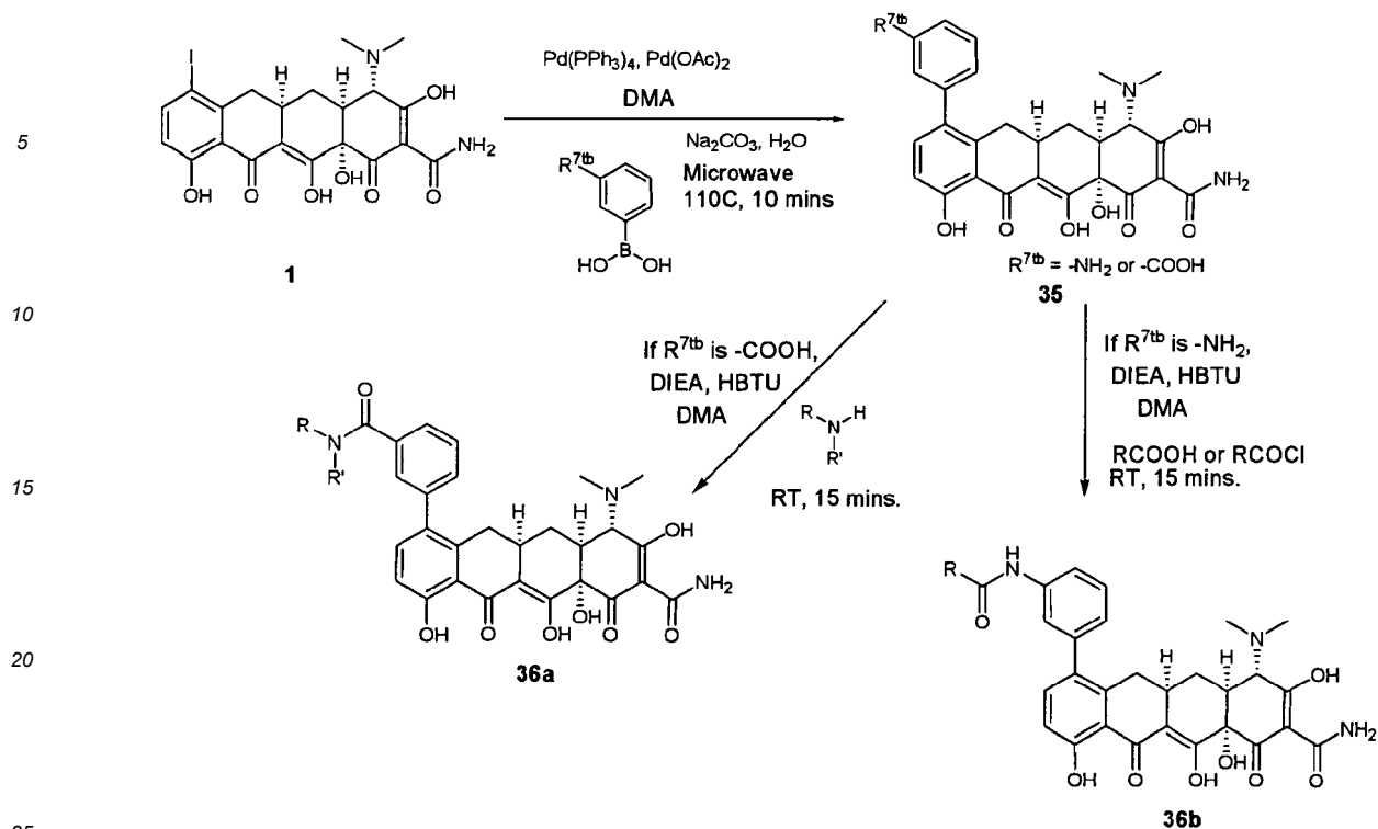
Scheme 16
