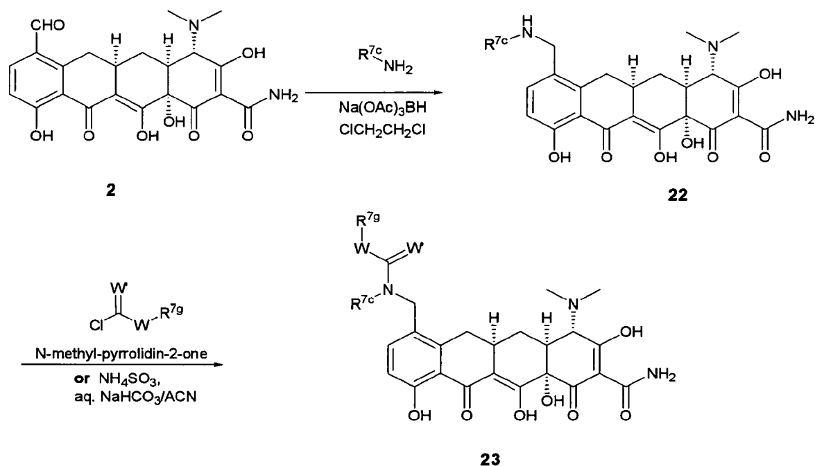
Scheme 10
