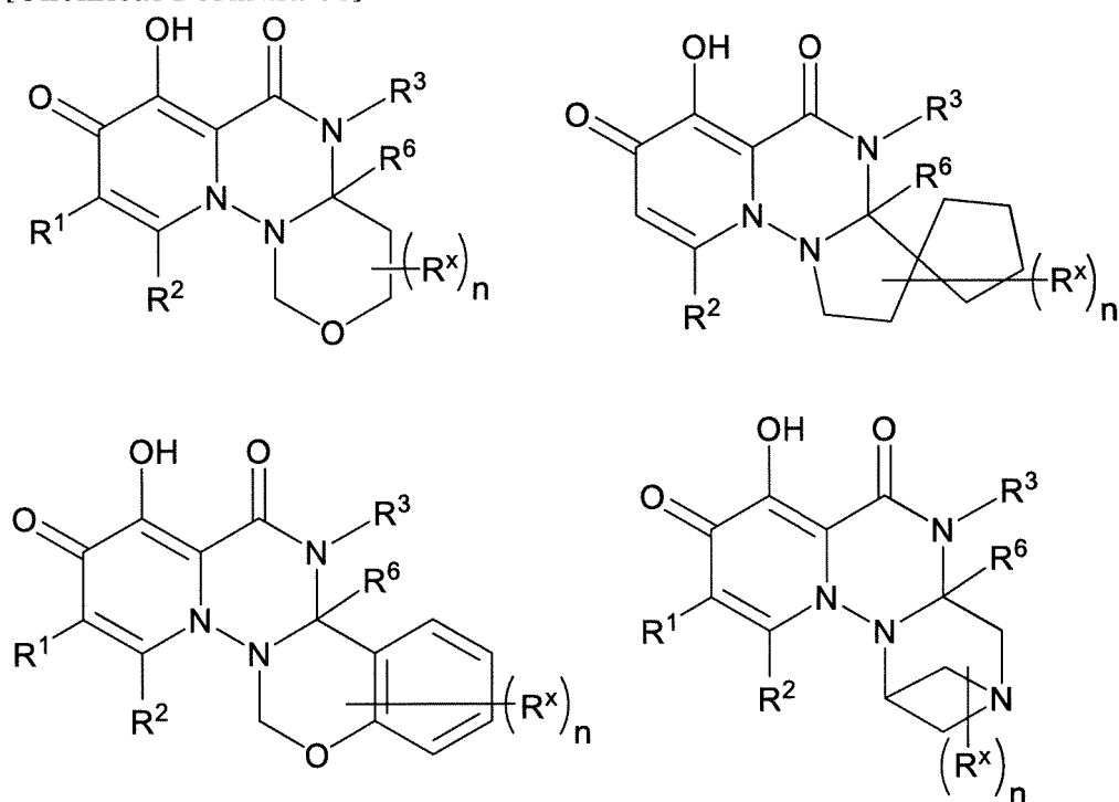
[Chemical Formula 38]
