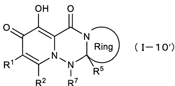
[Chemical Formula 40]
