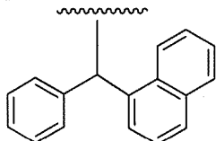
[Chemical Formula 18]
