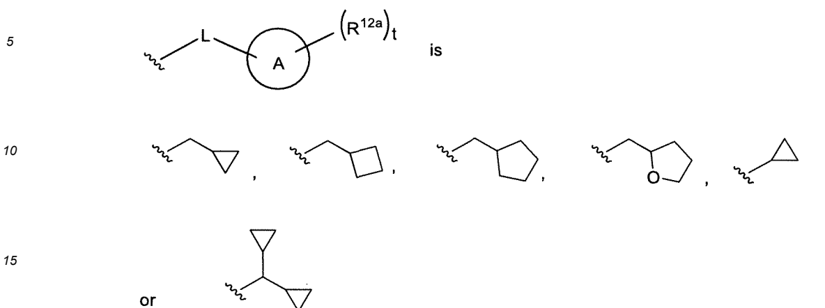
[Chemical Formula 74]
