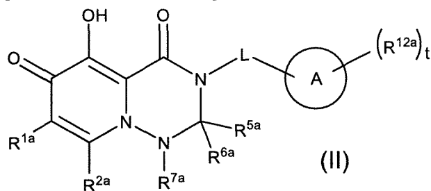
[Chemical Formula 4]
