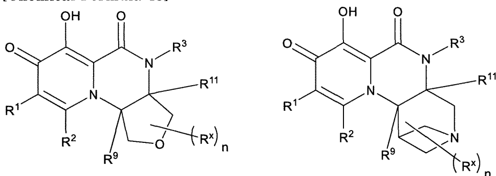
[Chemical Formula 43]
