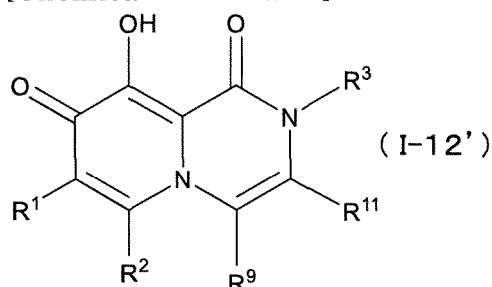
[Chemical Formula 44]
