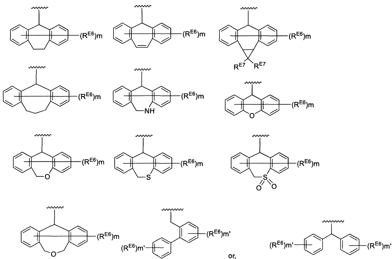
[Chemical Formula 2]
