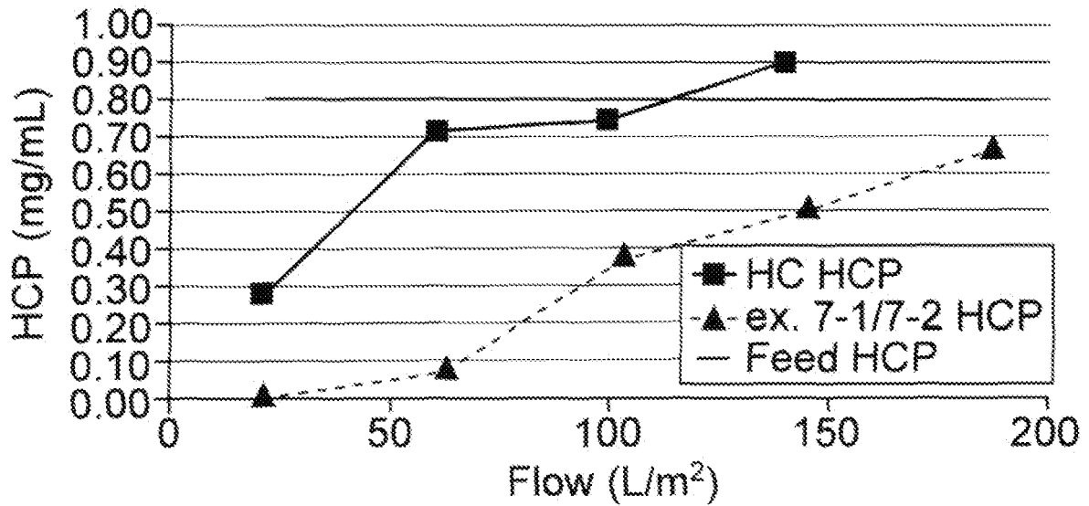
D0/X0 Coupled CHO-S mAb 05 HCP Breakthrough
