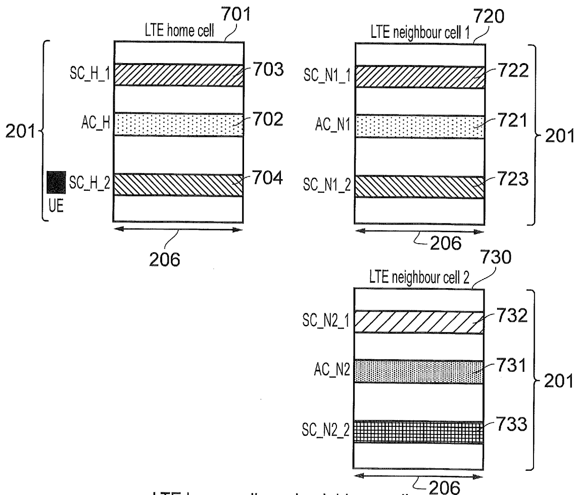
LTE home cells and neighbour cells
