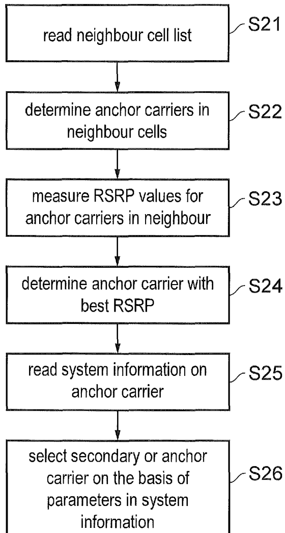
Flow chart of cell reselection process for when measurements are made on anchor carriers; and secondary carriers are listed in system information of the neighbour cell
