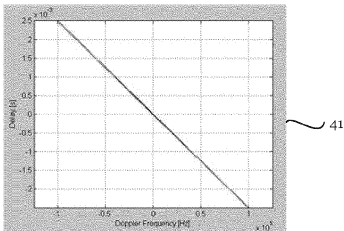
5ms pulse with chirp modulation
