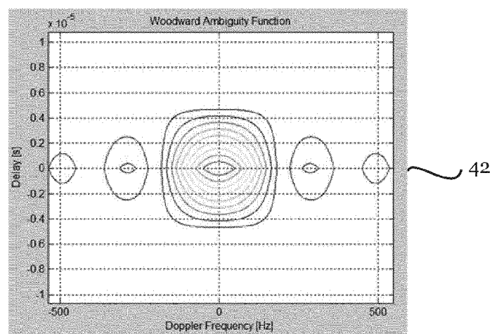
5ms pulse with PRN modulation
