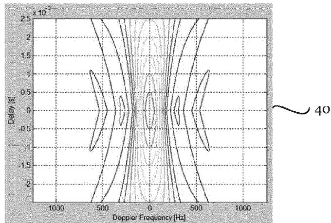
5ms pulse with no modulation
