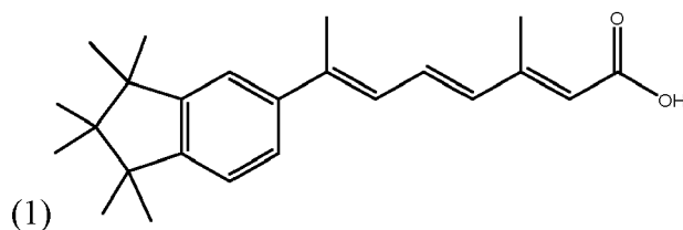
10 (2E,4E,6E)-7-(1,1,2,2,3,3-hexamethyl-2,3-dihydro-1H-inden-5-yl)-3-methylocta-2,4,6-trienoic acid or
