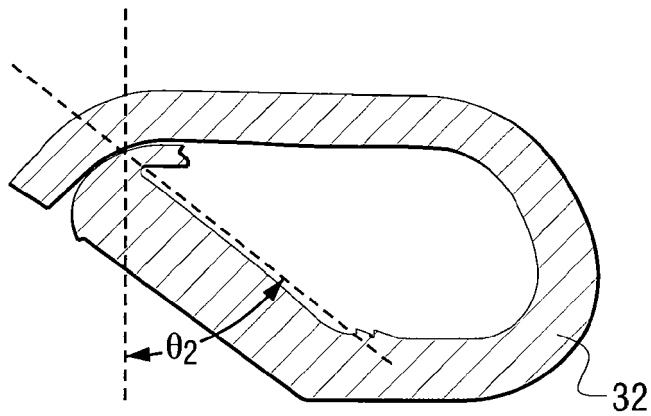
FIG. 5 PRIOR ART
