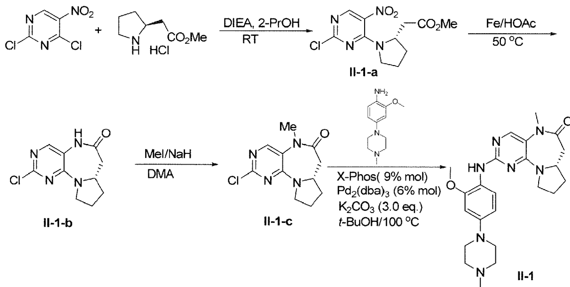
Scheme 2
