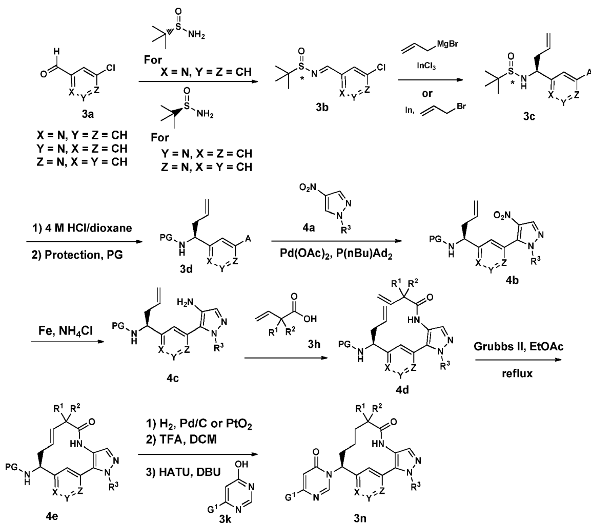
Scheme 4
