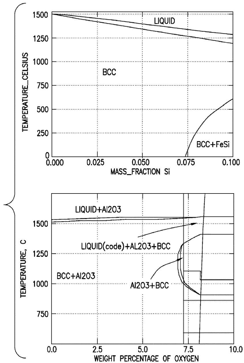
PHASE DIAGRAMS OF Fe-Al-Si ALLOY, (a) ISOPLETH OF Fe-9%Al-Si ALLOY SHOWING BCC STRUCTURE UP TO 1400C, (b) ISOPLETH OF Fe-9%Al-1%Si-O SHOWING PREFERENCE FOR FORMATION OF \text{Al}_2\text{O}_3
