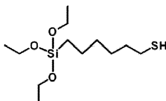
Compound 1-4'
