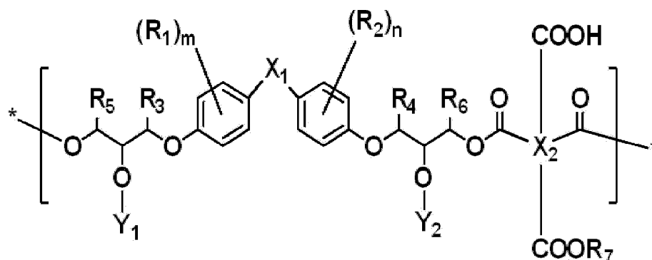
[Formula 1]
