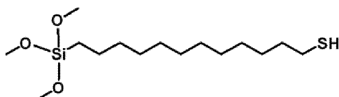
Compound 1-3'
