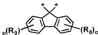
[Formula 2]
