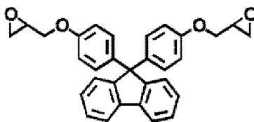
[Formula 6]
