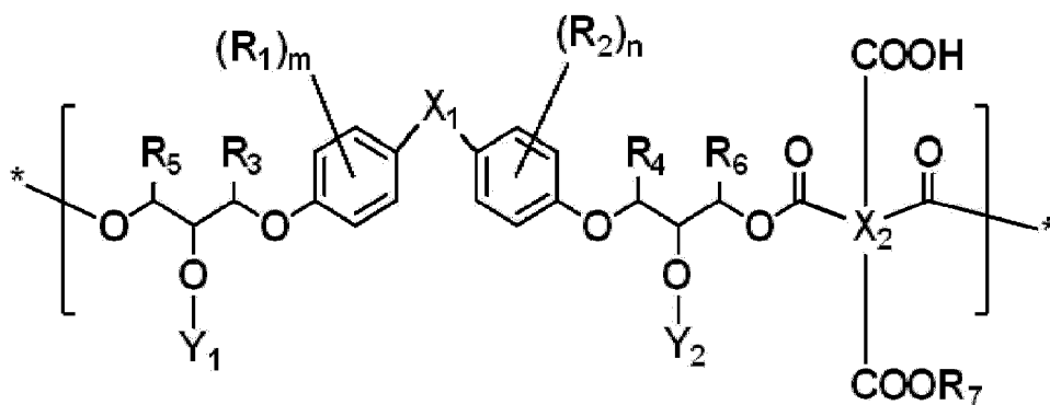
[Formula 1]
