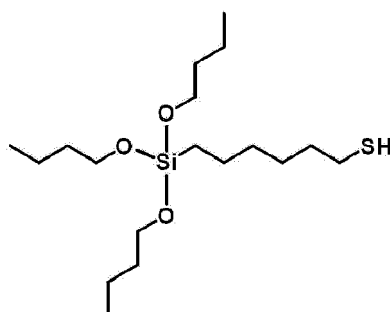
Compound 1-5'
