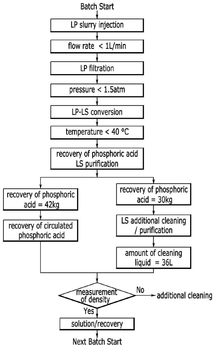
FIG. 9 &lt;LP-LS Automation of conversion process flow&gt;
