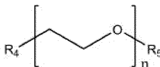
[Chemical Formula 3]
