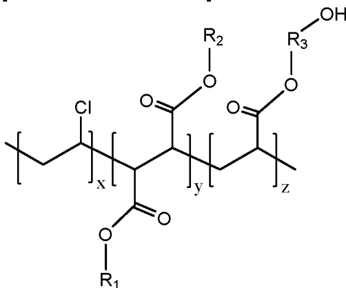
[Chemical Formula 2]
