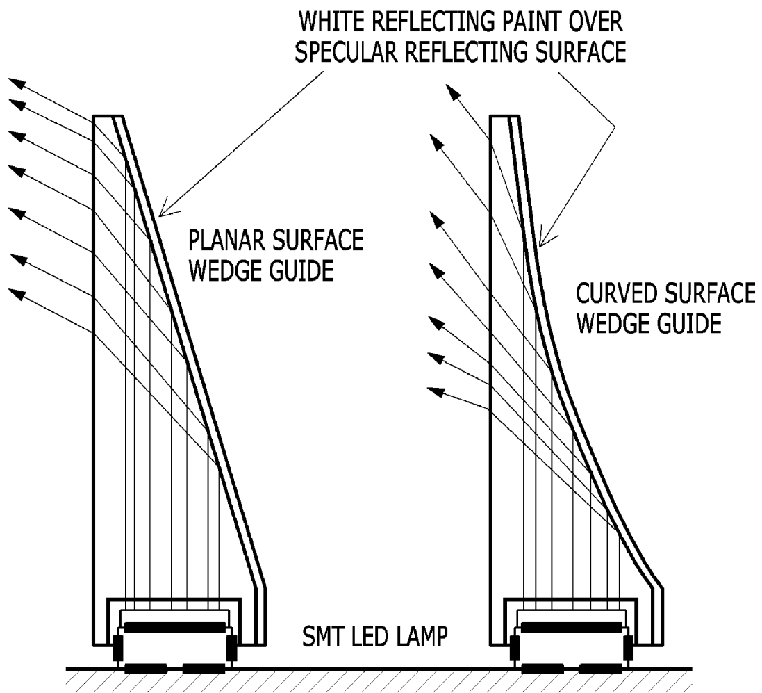
Wedge Light Guide(Side View)
