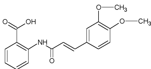
Tranilast
