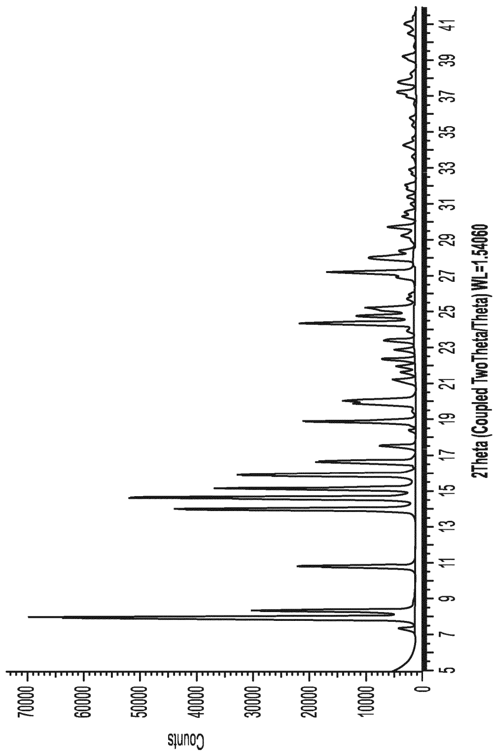
XRPD Pattern for the Crystalline 1:1 Tranilast N-methylglucamine Form II Salt
