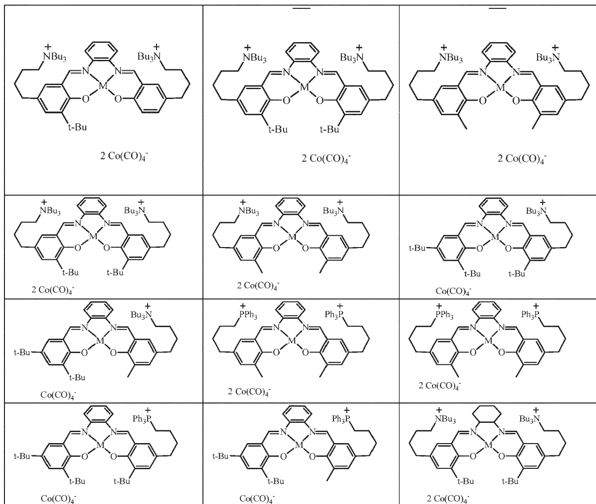
Catalyst Table 2
