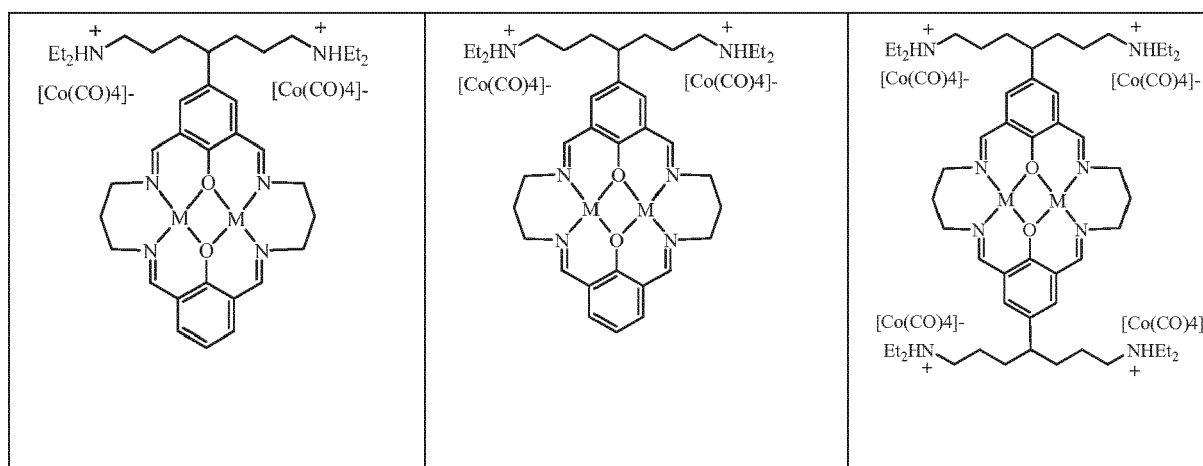
Catalyst Table 3
