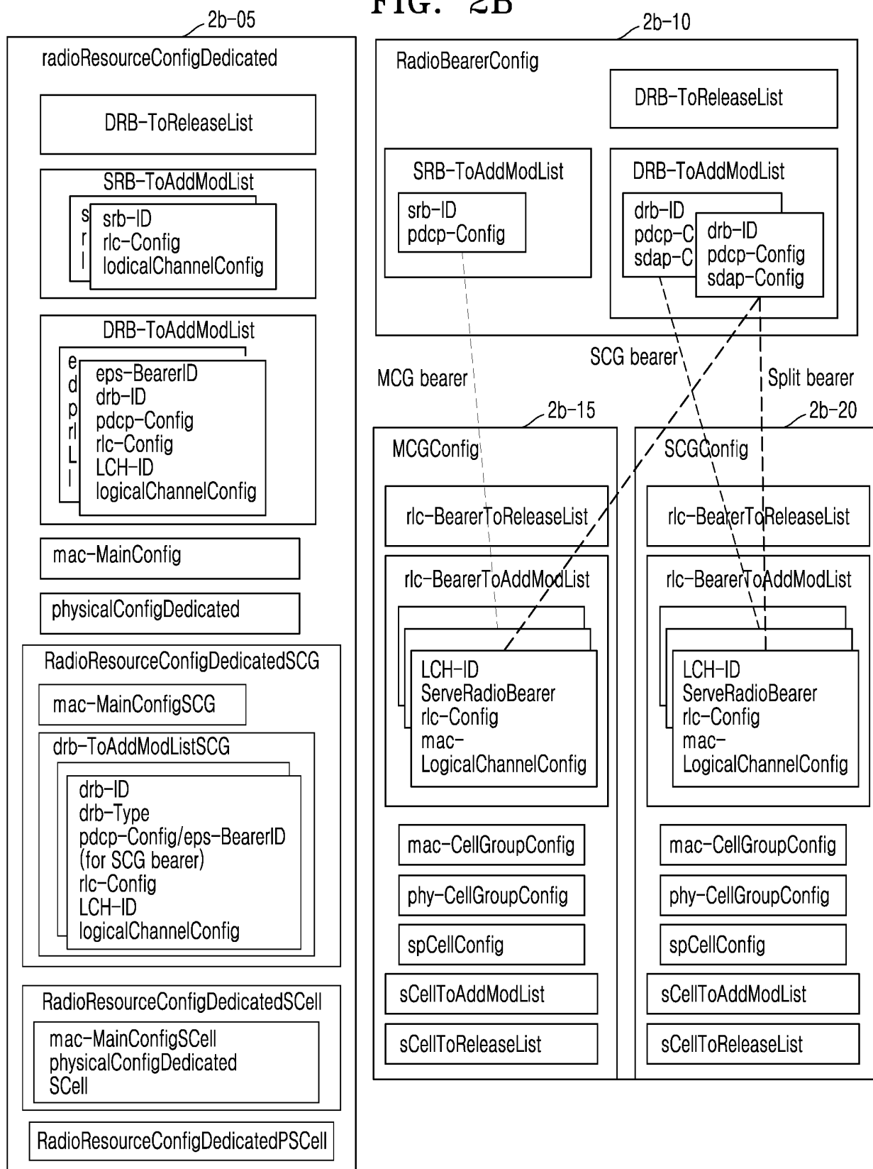
(a) RRCConnectionReconfiguration
