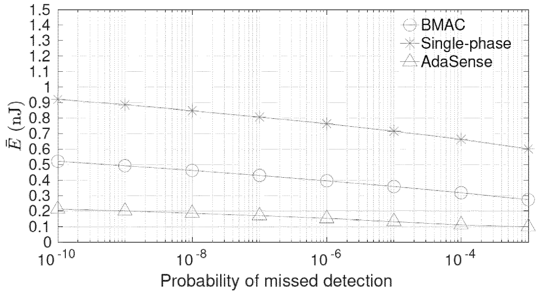
(a) n = 30 , P = -60\text{dBm} , P_{\text{FA}} = 10^{-3} . Energy savings 60%-63%.
