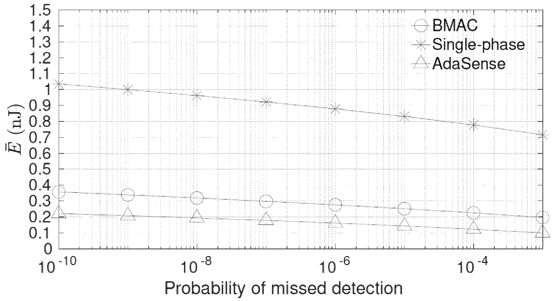
(c) n = 30 , P = -60\text{dBm} , P_{\text{FA}} = 10^{-5} . Energy savings 40%-50%.
