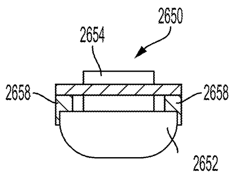
SECTION 43-43: UNDEFLECTED
