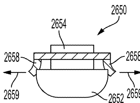
SECTION 43-43: DEFLECTED
