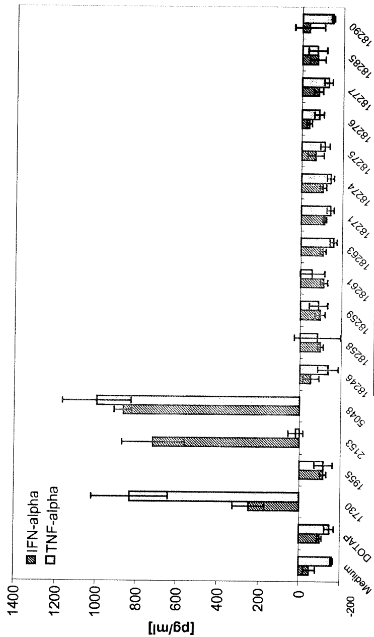
candidate siRNAs
