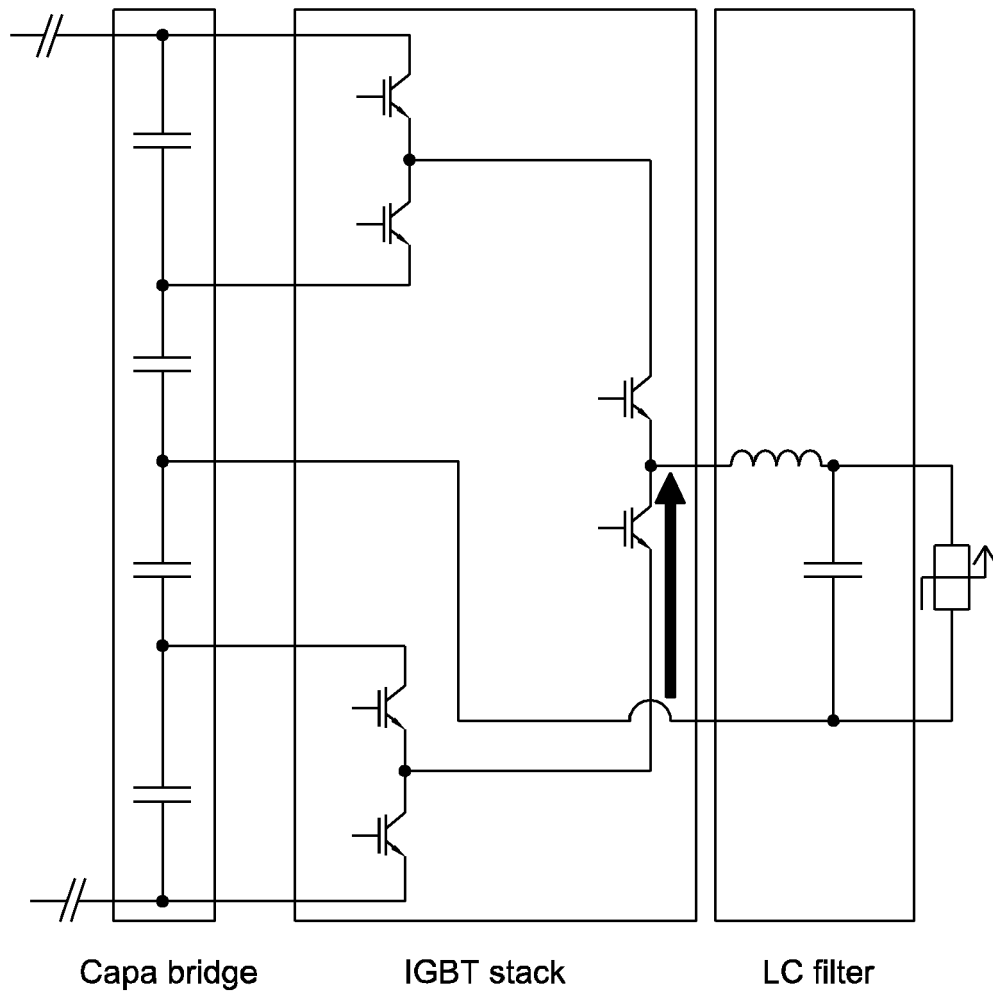
Dual-based 4-level Inverter Leg
