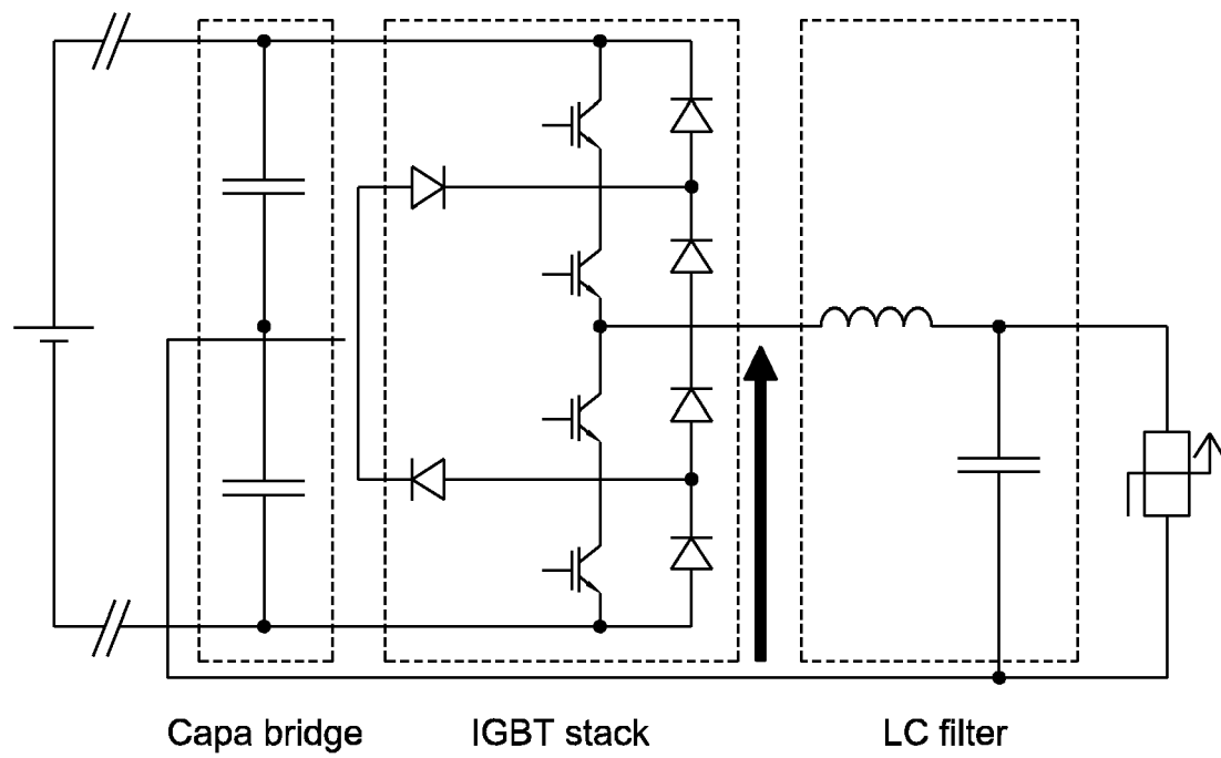
3-level NPC Inverter Leg
