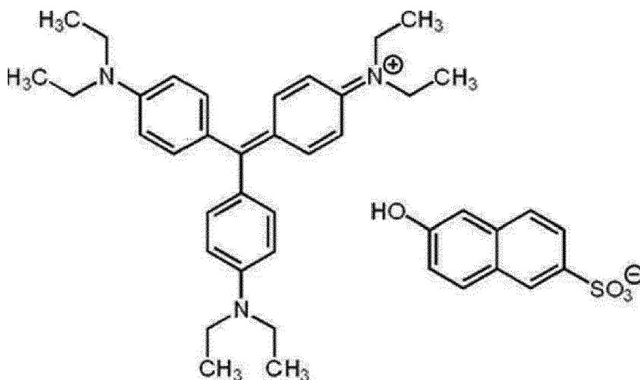
Ethyl violet
