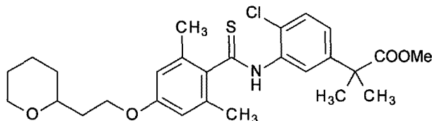
[Chemical 62]
