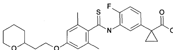
[Chemical 61]
