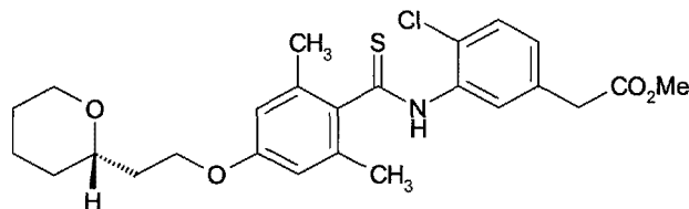
[Chemical 57]
