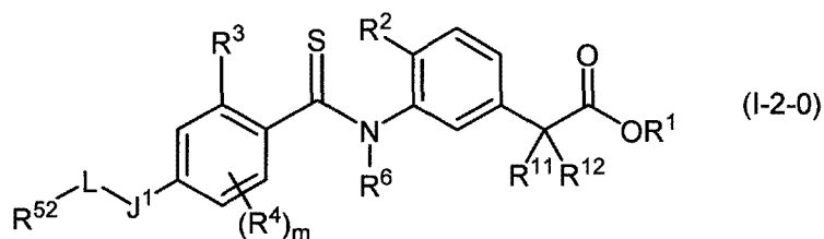
[Chemical 18]
