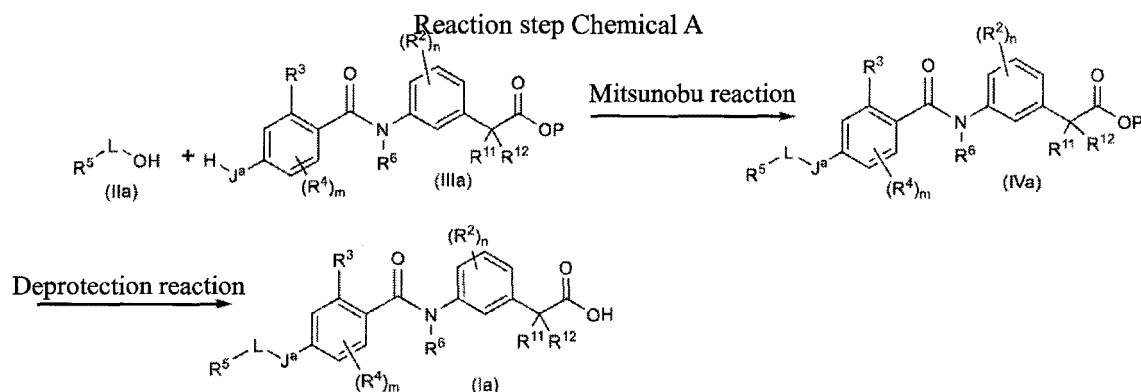
[Chemical 26]
