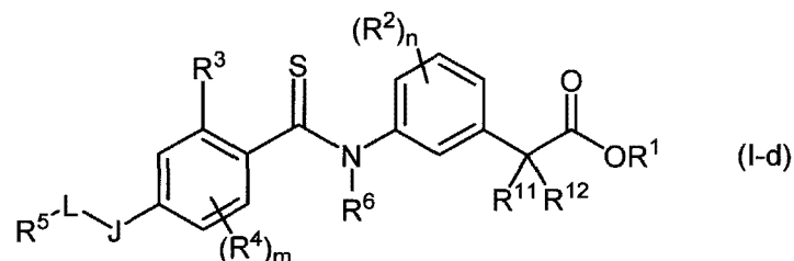
[Chemical 16]
