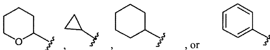
[Chemical 14]
