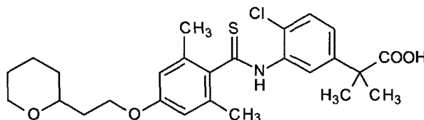
[Chemical 63]
