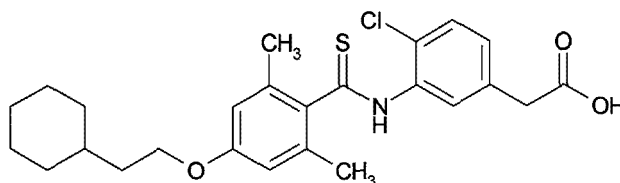
[Chemical 51]
