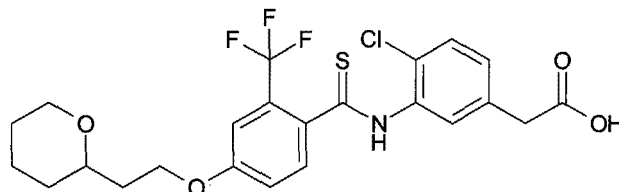
[Chemical 52]
