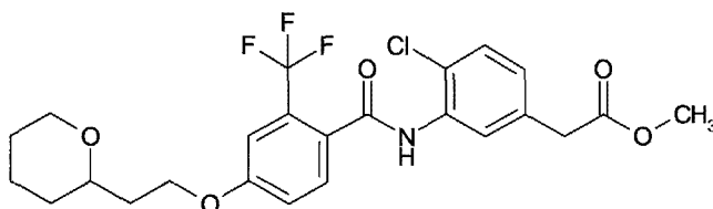
[Chemical 35]
