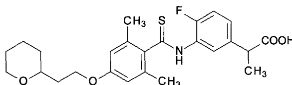
[Chemical 60]
