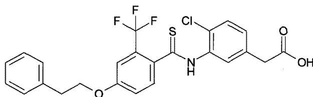
[Chemical 54]
