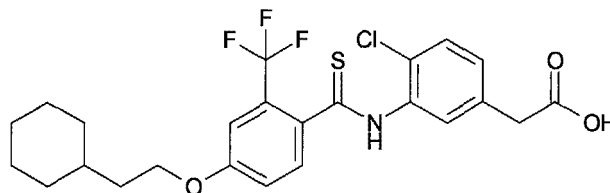
[Chemical 53]
