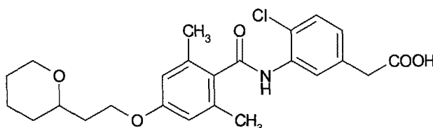
[Chemical 42]
