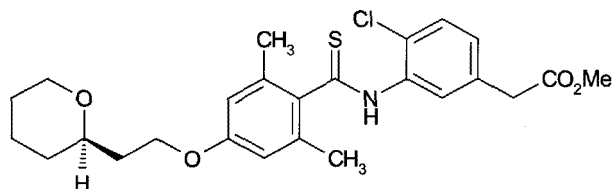
[Chemical 56]
