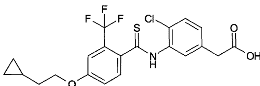
[Chemical 55]
