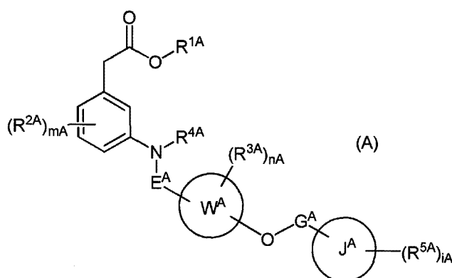
[Chemical 2]
