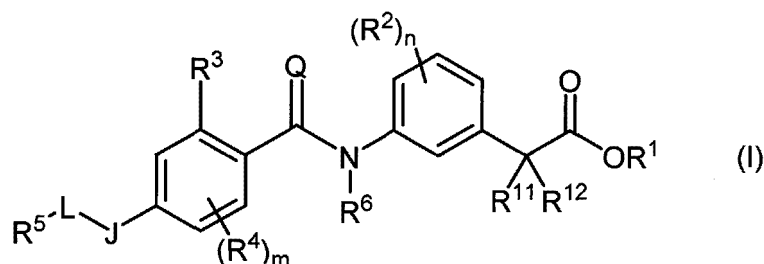
[Chemical 1]
