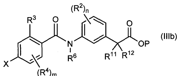
[Chemical 29]
