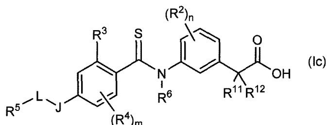
[Chemical 31]
