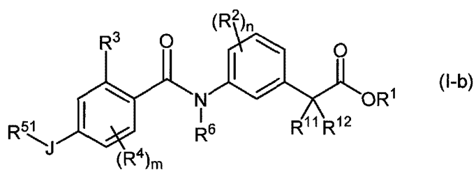
[Chemical 10]
