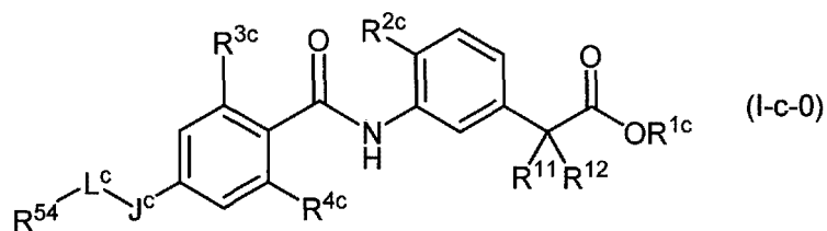
[Chemical 11]
