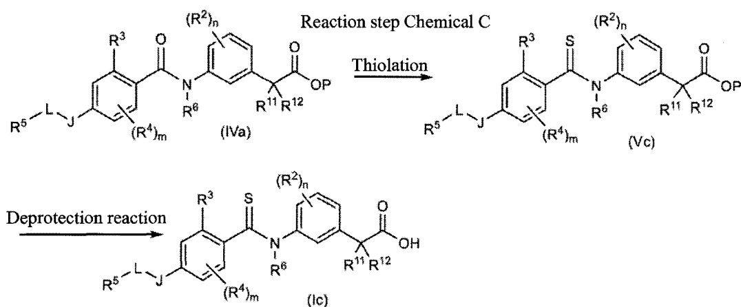
[Chemical 32]
