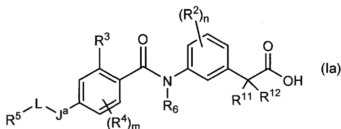
[Chemical 25]
