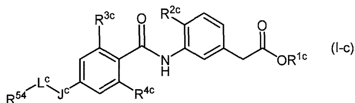
[Chemical 15]
