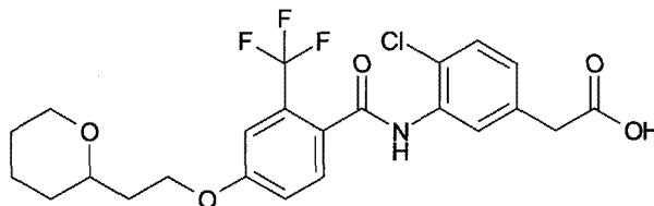
[Chemical 36]
