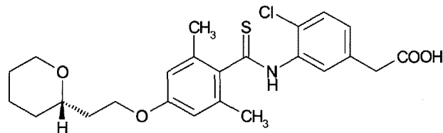
[Chemical 59]
