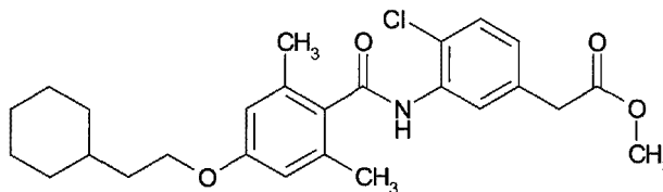
[Chemical 41]
