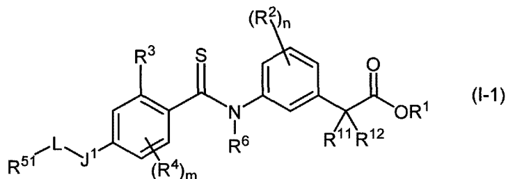
[Chemical 17]
