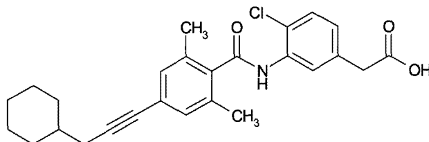
[Chemical 47]
