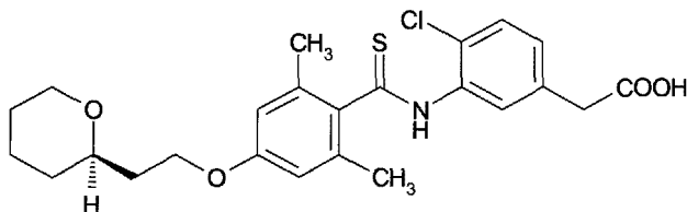
[Chemical 58]
