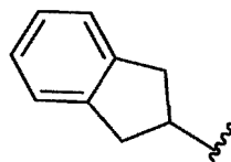
[Chemical 12]
