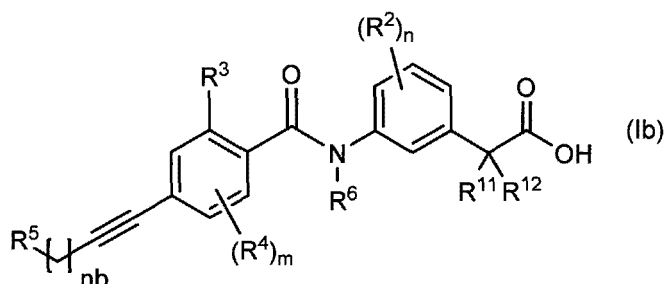
[Chemical 28]
