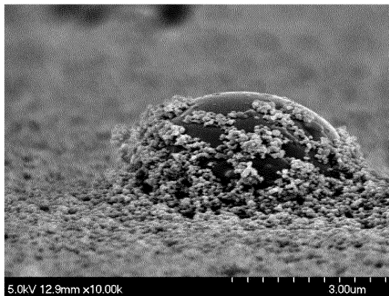
FIG.8 SEM image of Example 5
