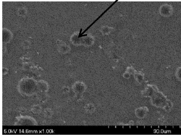
FIG.6 SEM image of Example 2
