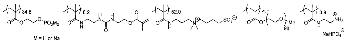
Compound for undercoat layer (UC-2)
