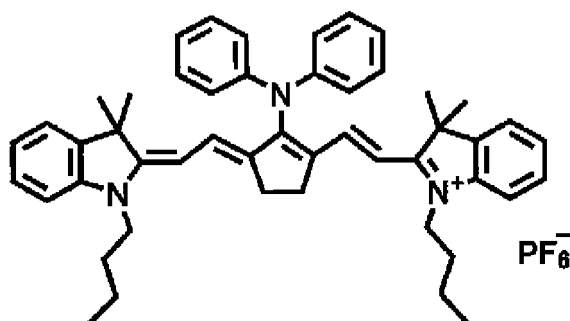
Infrared absorbent 4
