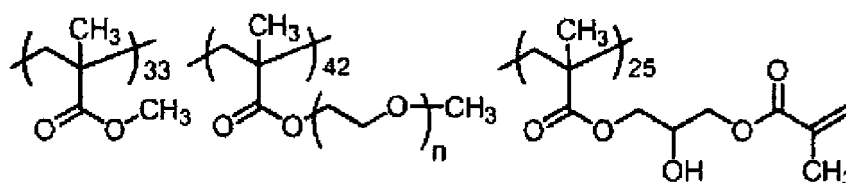
Binder polymer (2)
