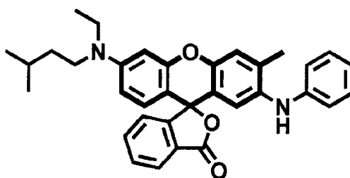
Printing-out agent
