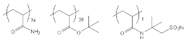
Hydrophilic polymer (1)
