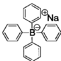
Borate compound (1)
