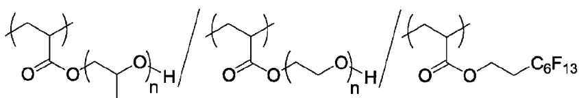
Fluorine-based surfactant
