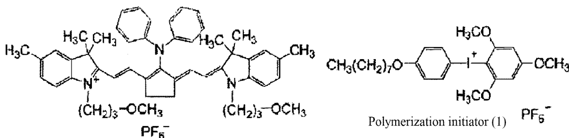
Infrared absorbent (1)
