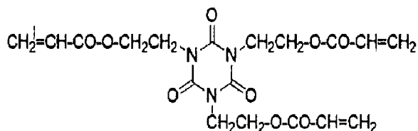
Polymerizable compound (1)
