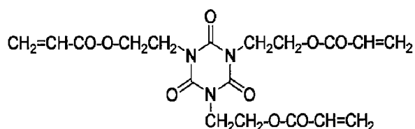
Polymerizable compound (1)
