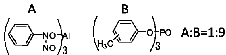
Mercapto compound
