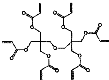
Polymerizable compound (2)
