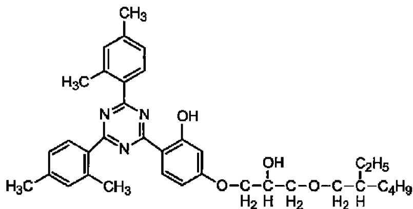
Ultraviolet absorbent (1)
