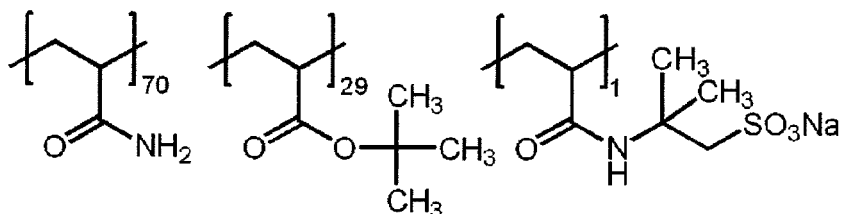
Hydrophilic polymer (2)
