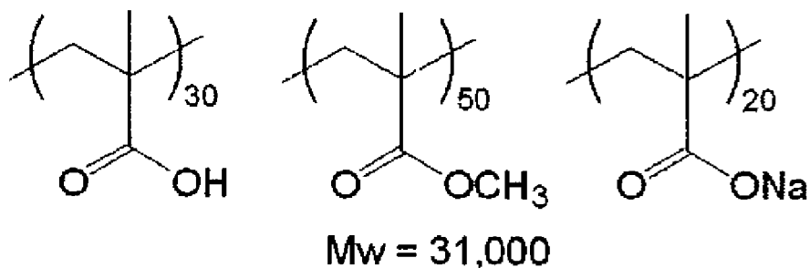
Polymer U
