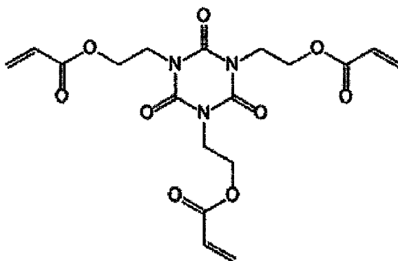
Polymerizable compound (1)
