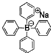
Borate compound (1)
