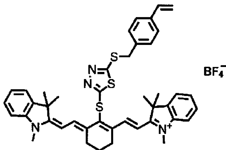
Infrared absorbent 1
