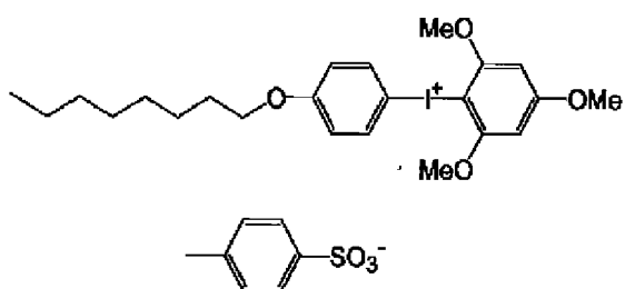
Polymerization initiator 1
