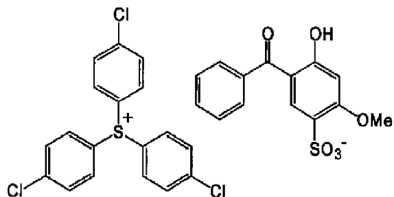
Polymerization initiator 2
