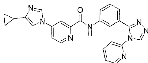
4-(4-cyclopropyl-1H-imidazol-1-yl)-N-(3-(4-(pyridin-2-yl)-4H-1,2,4-triazol-3-yl)phenyl)picolinamide;
