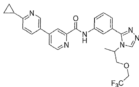
6-cyclopropyl-N-(3-(4-(1-(2,2,2-trifluoroethoxy)propan-2-yl)-4H-1,2,4-triazol-3-yl)phenyl)-3,4'-bipyridine-2'-carboxamide;
