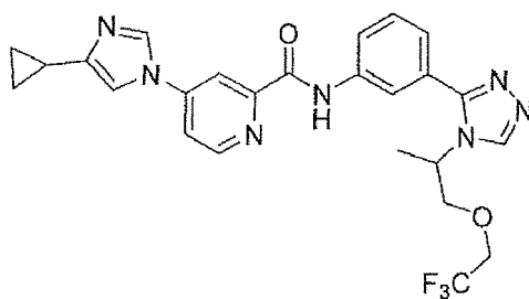
4-(4-cyclopropyl-1H-imidazol-1-yl)-N-(3-(4-(1-(2,2,2-trifluoroethoxy)propan-2-yl)-4H-1,2,4-triazol-3-yl)phenyl)picolinamide
