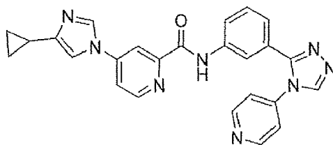
4-(4-cyclopropyl-1H-imidazol-1-yl)-N-(3-(4-(pyridin-4-yl)-4H-1,2,4-triazol-3-yl)phenyl)picolinamide;
