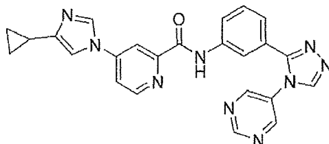
4-(4-cyclopropyl-1H-imidazol-1-yl)-N-(3-(4-(pyrimidin-5-yl)-4H-1,2,4-triazol-3-yl)phenyl)picolinamide;
