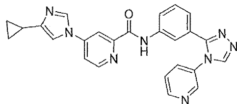
4-(4-cyclopropyl-1H-imidazol-1-yl)-N-(3-(4-(pyridin-3-yl)-4H-1,2,4-triazol-3-yl)phenyl)picolinamide;
