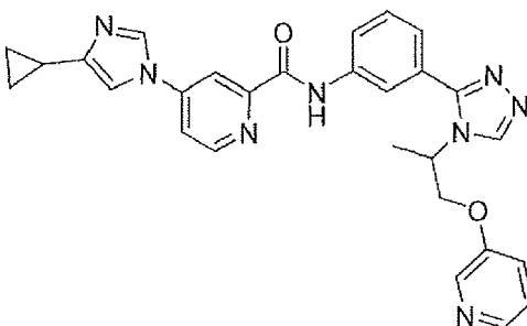
4-(4-cyclopropyl-1H-imidazol-1-yl)-N-(3-(4-(1-(pyridin-3-yloxy)propan-2-yl)-4H-1,2,4-triazol-3-yl)phenyl)picolinamide and
