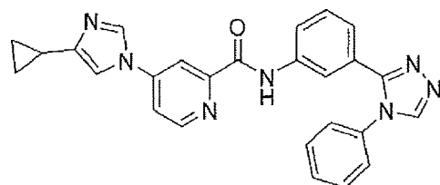
4-(4-cyclopropyl-1H-imidazo1-1-yl)-N-(3-(4-phenyl-4H-1,2,4-triazol-3-yl)phenyl)picolinamide;
