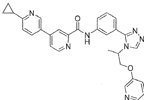
6-cyclopropyl-N-(3-(4-(1-(pyridin-3-yloxy)propan-2-yl)-4H-1,2,4-triazol-3-yl)phenyl)-3,4'-bipyridine-2'-carboxamide;
