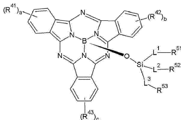
[Chemical Formula 10]
