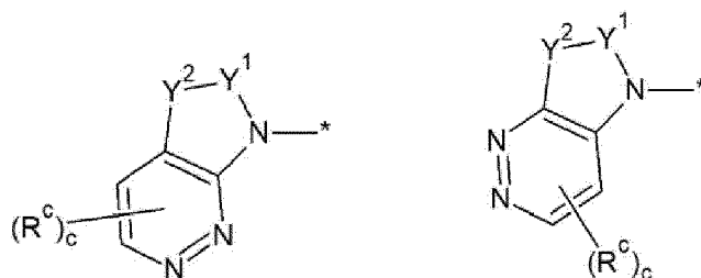
[Chemical Formula 2A-9]
