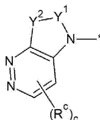
[Chemical Formula 2A-10]
