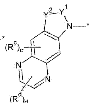
[Chemical Formula 2B-9]
