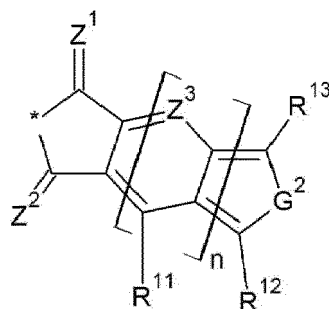
[Chemical Formula 4E]
