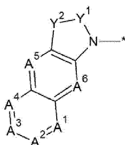
[Chemical Formula 2B]
