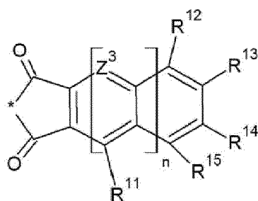
[Chemical Formula 4A-2]
