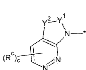
[Chemical Formula 2A-9]
