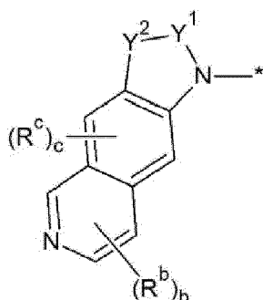
[Chemical Formula 2B-4]
