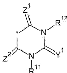
[Chemical Formula 4B]
