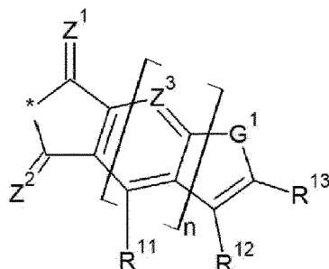
[Chemical Formula 4D]
