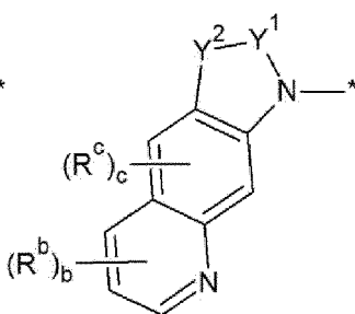
[Chemical Formula 2B-4]
