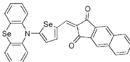
[Reaction Scheme 2-1]
