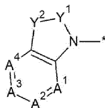
[Chemical Formula 2A]
