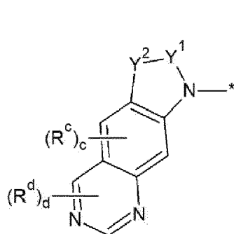
[Chemical Formula 2B-9]
