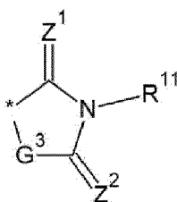
[Chemical Formula 4F]
