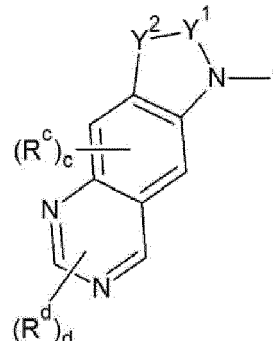
[Chemical Formula 2B-10]
