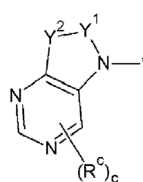
[Chemical Formula 2A-8]
