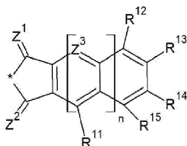
[Chemical Formula 4A]
