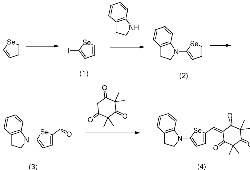
[Reaction Scheme 1-1]
