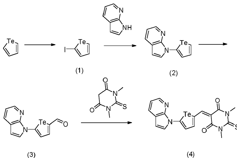
[Reaction Scheme 1-5]
