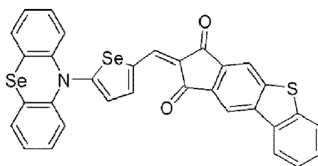
[Chemical Formula 2-2]
