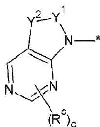
[Chemical Formula 2A-6]
