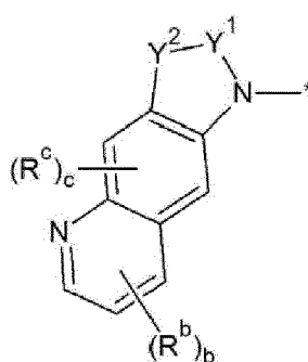
[Chemical Formula 2B-5]
