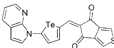
[Reaction Scheme 1-5]
