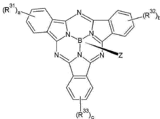
[Chemical Formula 7]
