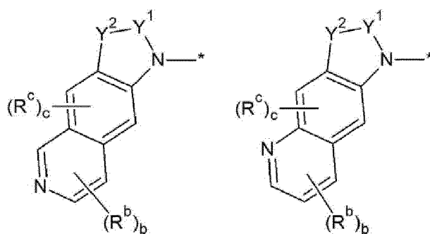
[Chemical Formula 2B-4]
