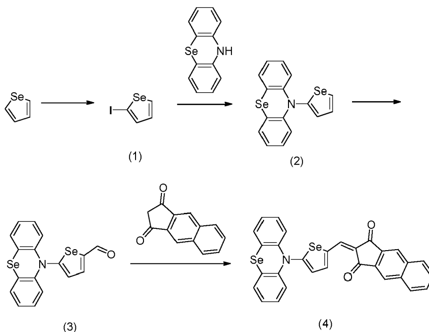
[Reaction Scheme 2-1]
