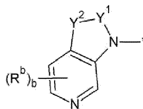
[Chemical Formula 2A-5]
