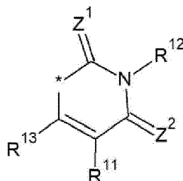
[Chemical Formula 4C]
