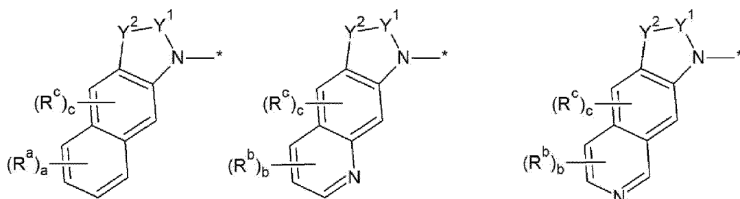
[Chemical Formula 2B-4]
