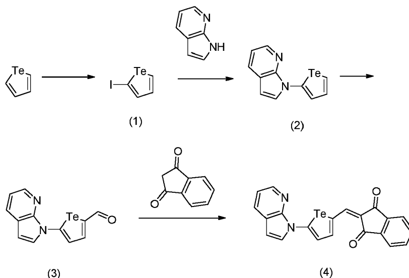
[Reaction Scheme 1-2]
