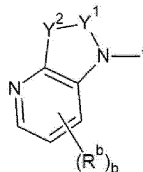
[Chemical Formula 2A-5]
