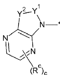
[Chemical Formula 2A-7]
