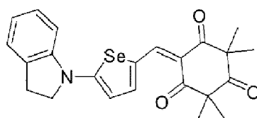
[Reaction Scheme 1-1]
