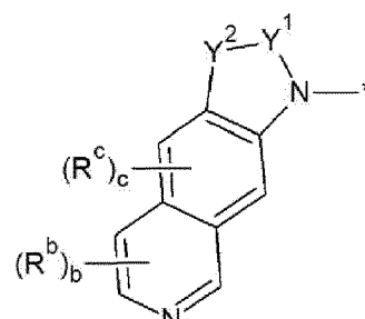
[Chemical Formula 2B-5]
