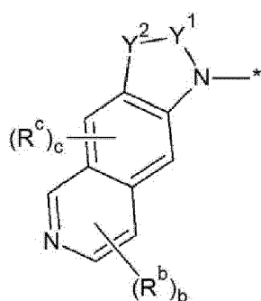
[Chemical Formula 2B-4]
