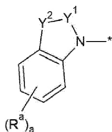
[Chemical Formula 2A-1]
