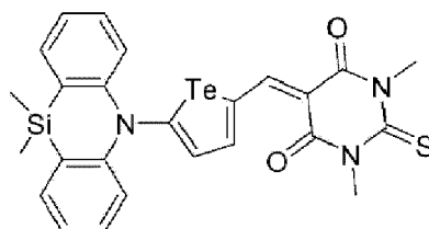
[Reaction Scheme 2-4]
