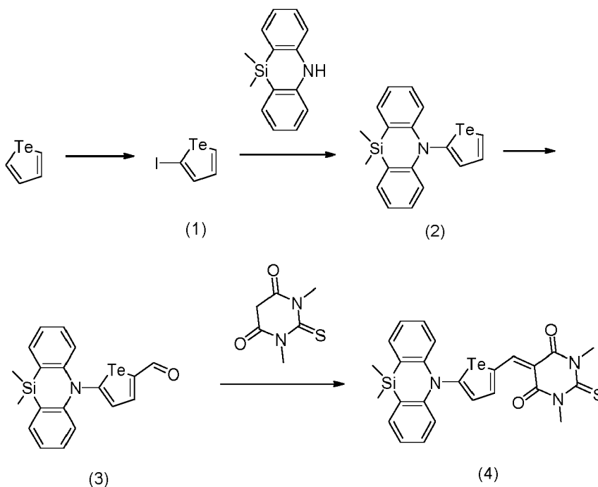
[Reaction Scheme 2-4]
