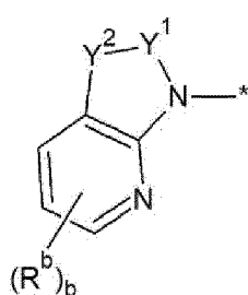
[Chemical Formula 2A-2]
