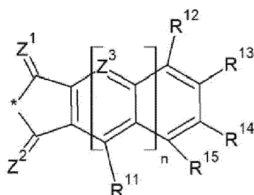
[Chemical Formula 4A]
