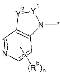
[Chemical Formula 2A-4]
