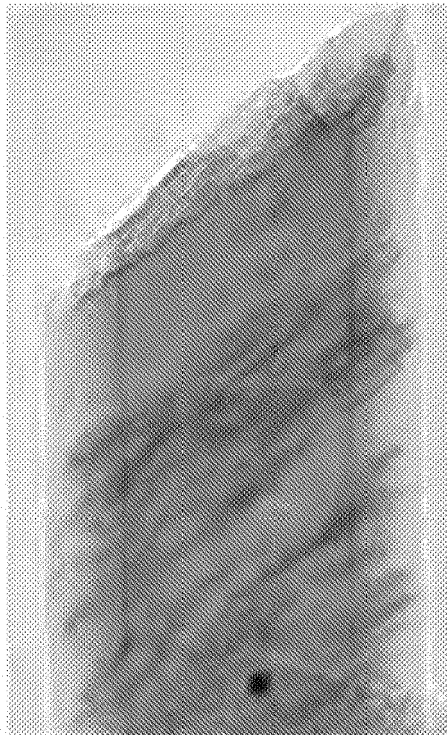
Low-X-Ray Density Regions in a diamond FIG. 6
