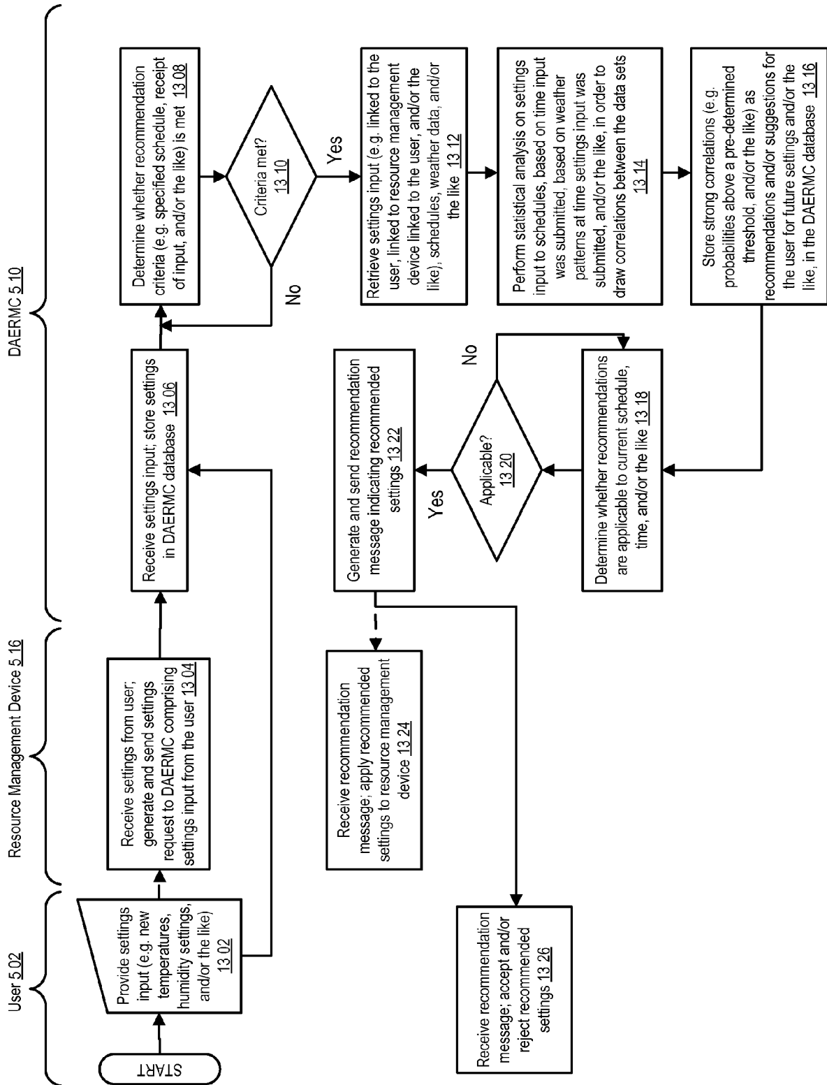
Resource Usage Recommendation Component
