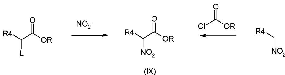
Reaction scheme 6:
