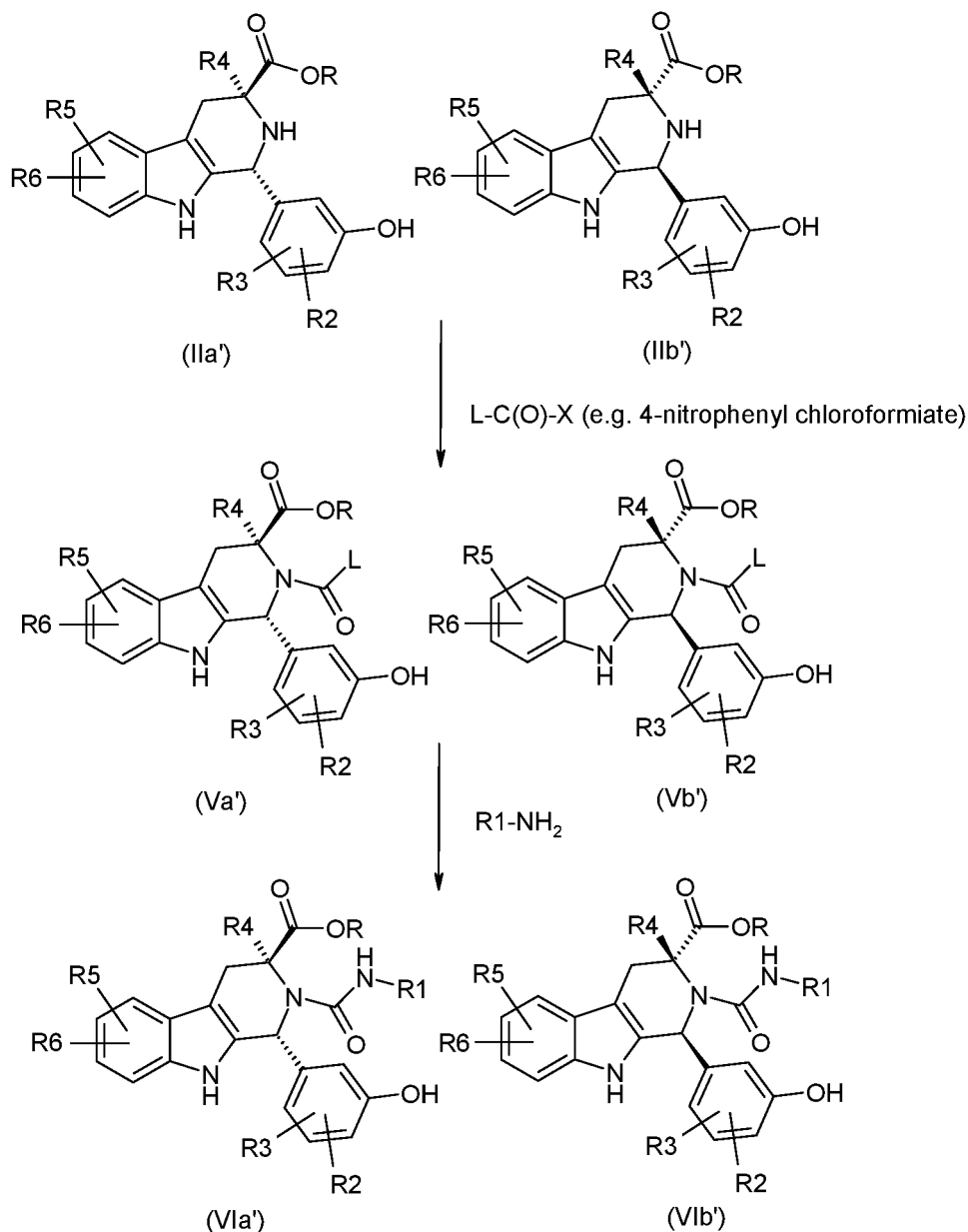
Reaction scheme 4:
