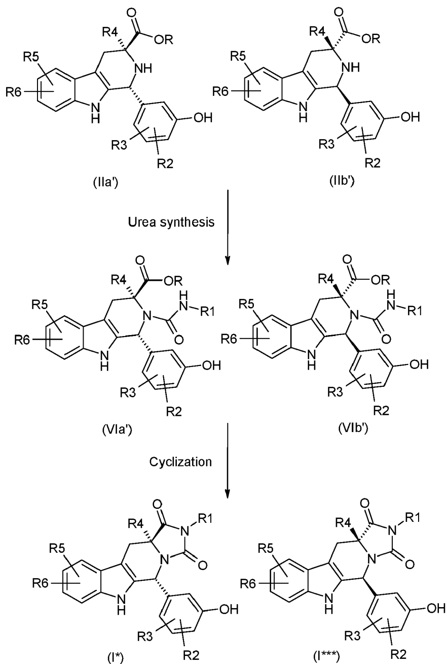
Reaction scheme 3:
