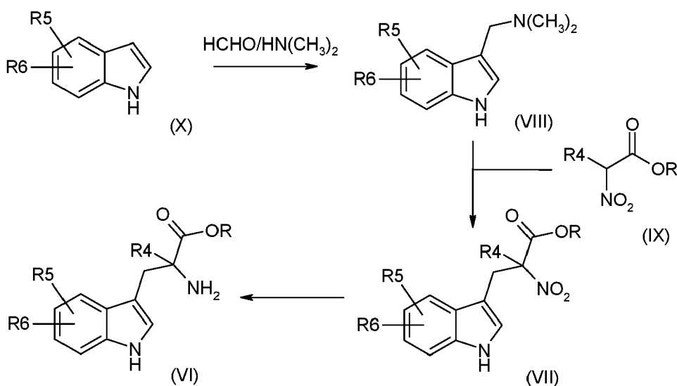
Reaction scheme 5:
