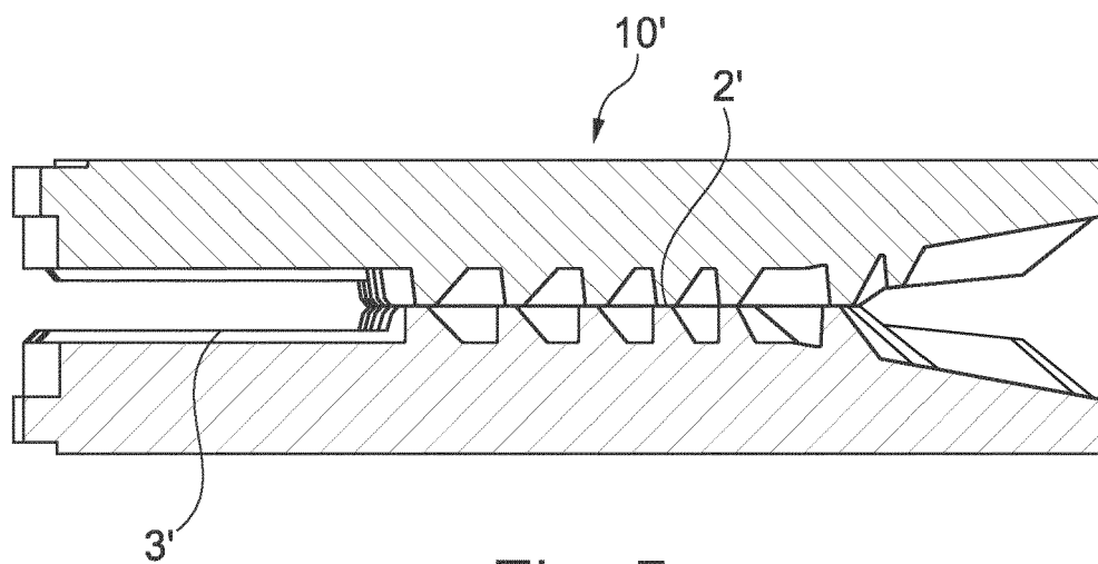
Fig. 5 PRIOR ART
