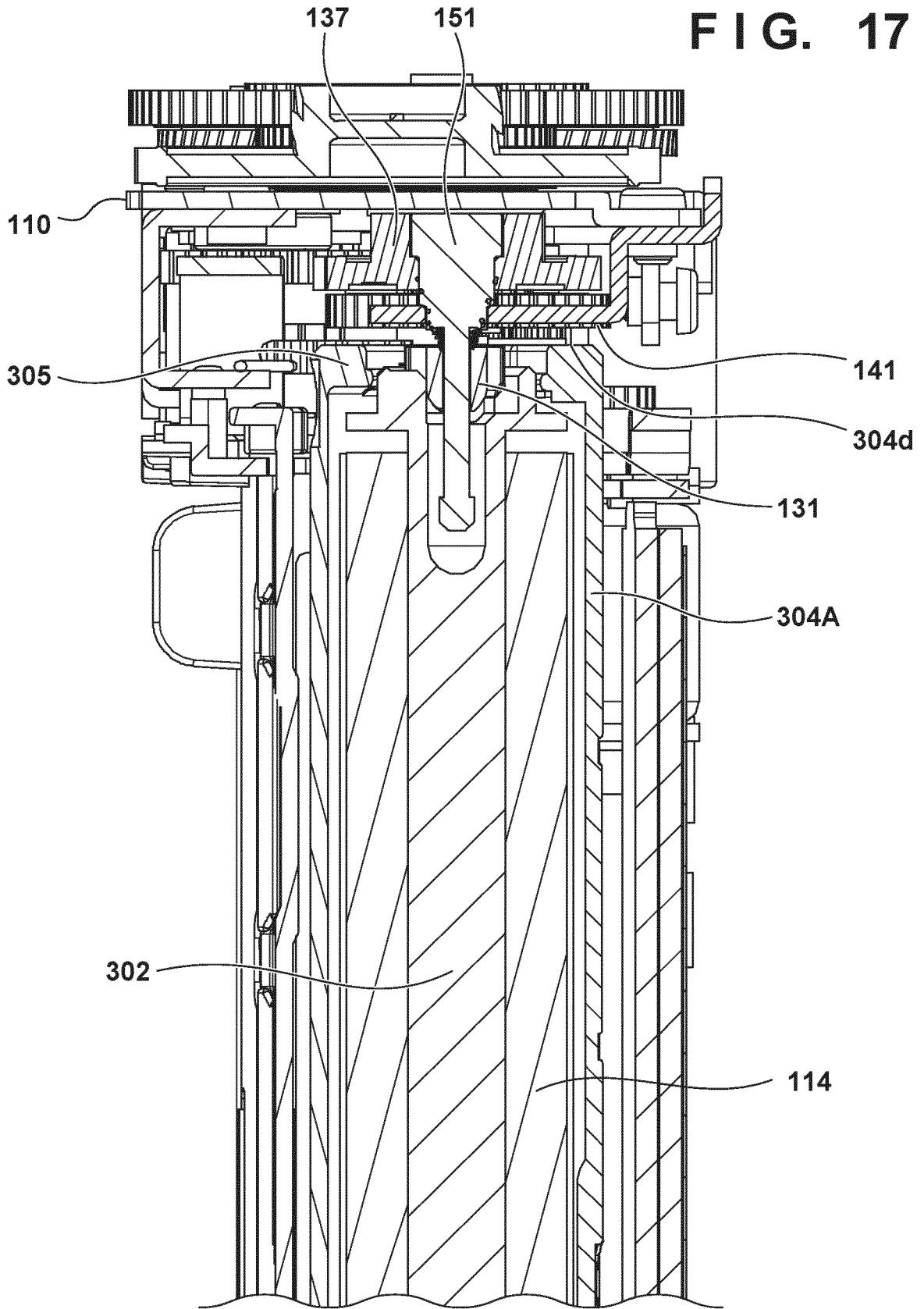
V-V CROSS SECTION
