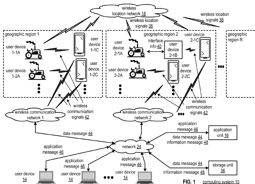
FIG. 1 computing system 10
