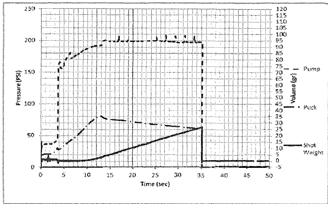
Graph 3 Grinder at -60
