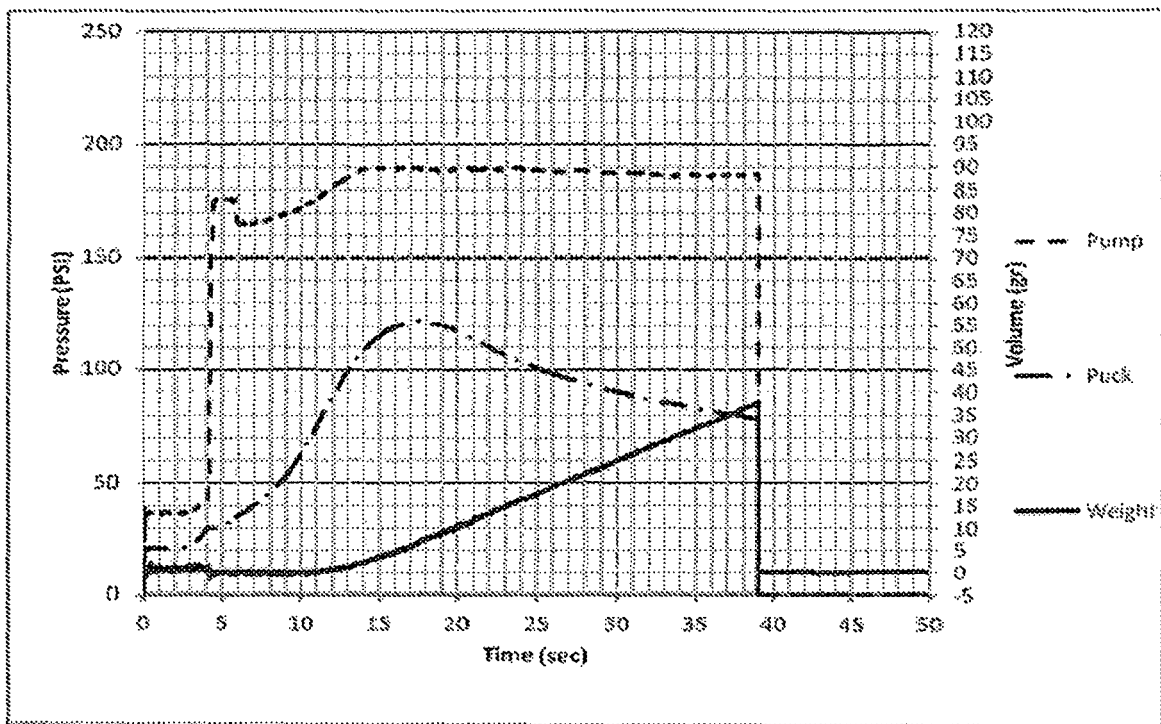
Graph 9: 38.9 gram shot
