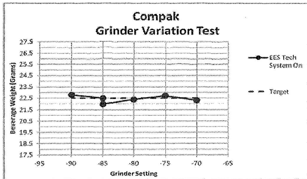
Graph 6: 22.5 gram shot
