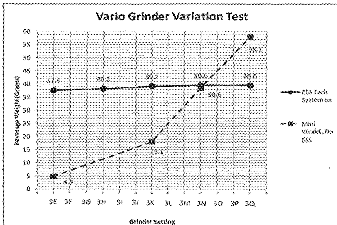
Graph 5: 38.9 gram shot
