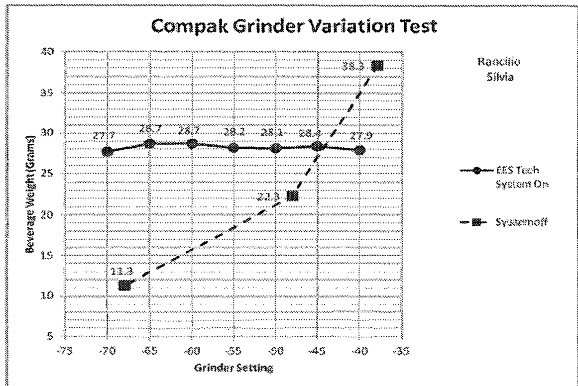
Graph 4: 28.5 gram shot
