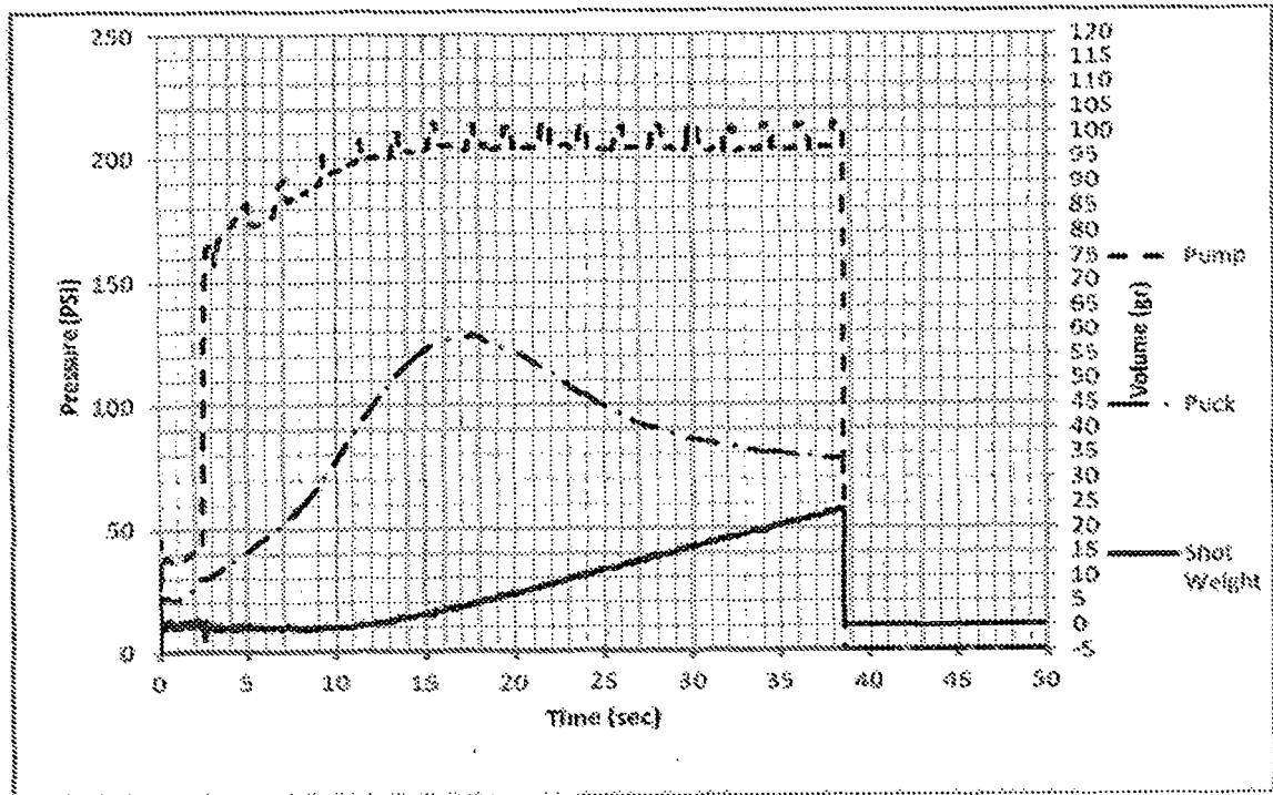
Graph 10: 22.5 gram shot
