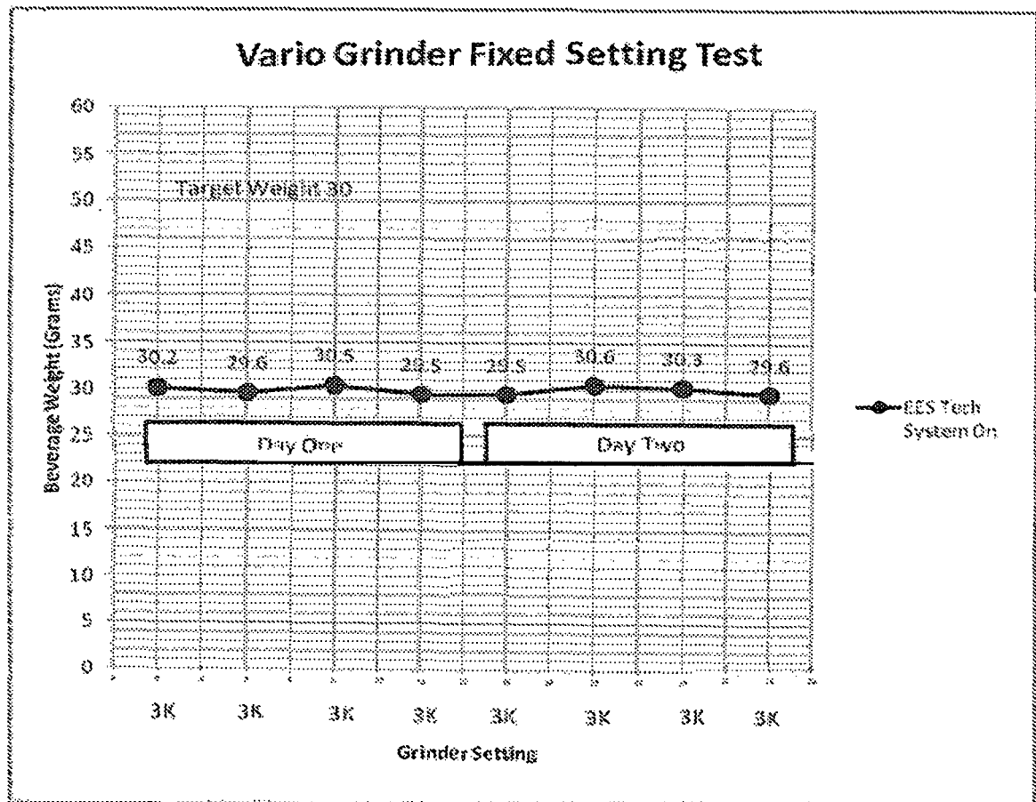
Graph 12: Repeatability of system shot weight
