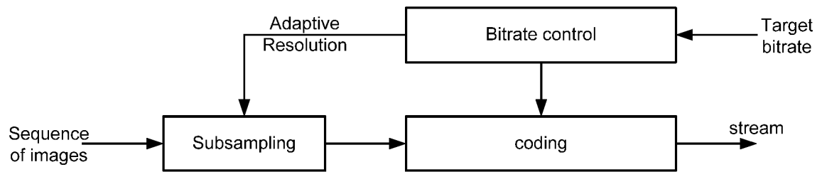
FIGURE 1 – PRIOR ART
