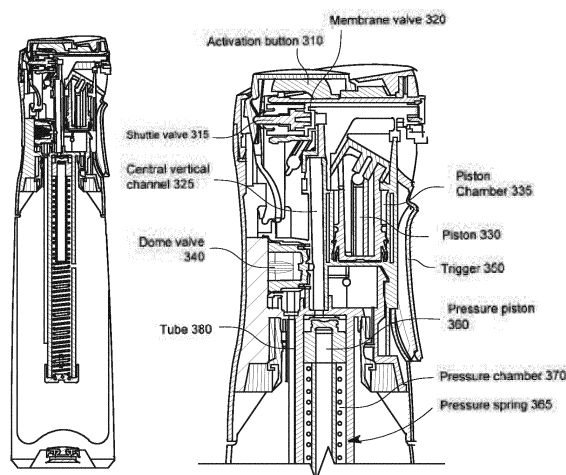
Fig. 3 - Flairosol With Activation Button
