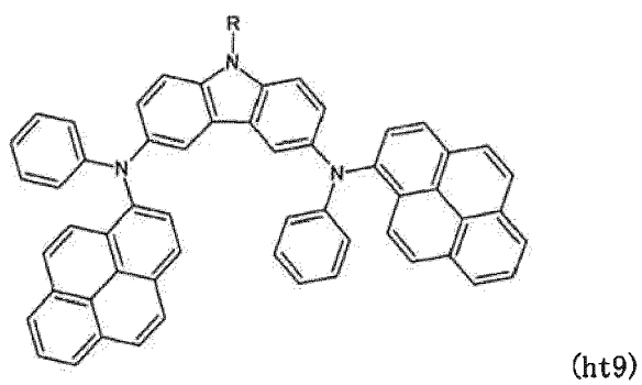
[Chemical formula 84]
