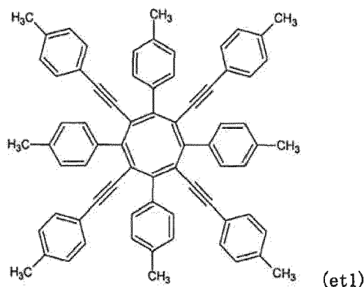
[Chemical formula 171]
