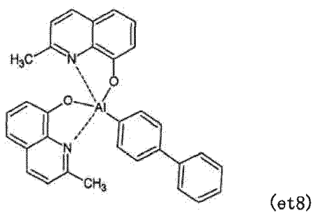
[Chemical formula 178]
