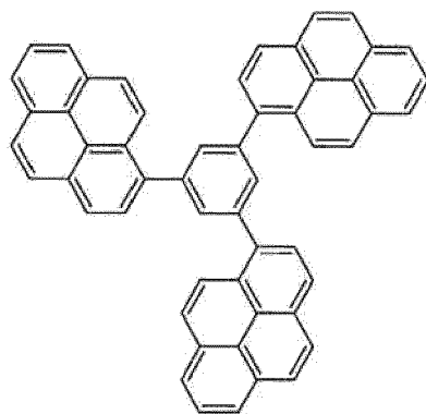
[Chemical formula 152]
