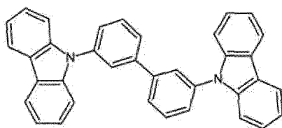
[Chemical formula 211]
