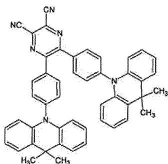
[Chemical formula 212]
