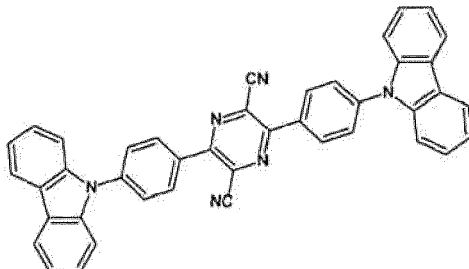
[Chemical formula 219]
