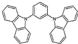
[Chemical formula 210]
