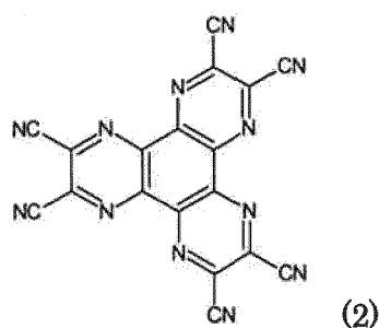
[Chemical formula 3]
