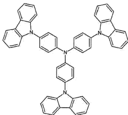
[Chemical formula 91]
