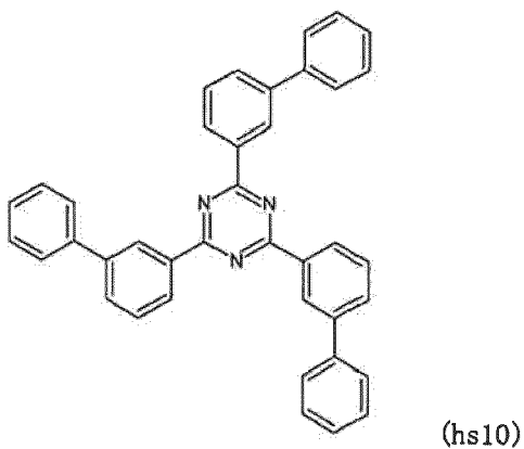
[Chemical formula 169]
