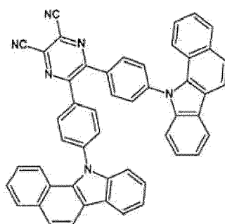
(BCz-CNP)
