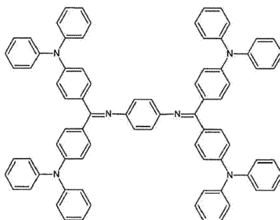
[Chemical formula 111]
