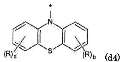
[Chemical formula 19]
