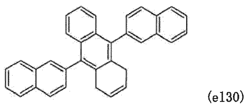
[Chemical formula 149]
