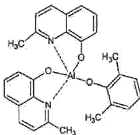
[Chemical formula 176]
