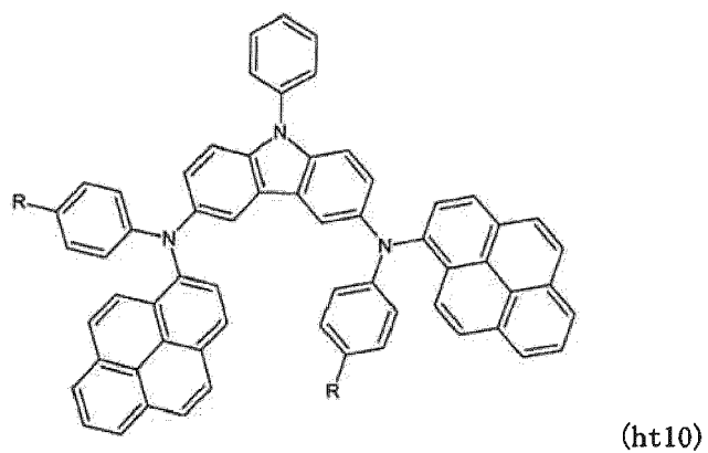
[Chemical formula 86]
