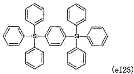
[Chemical formula 144]
