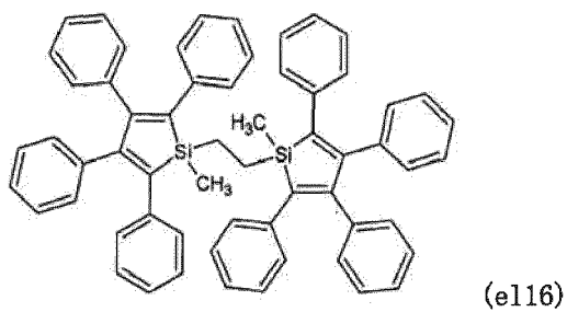
[Chemical formula 135]
