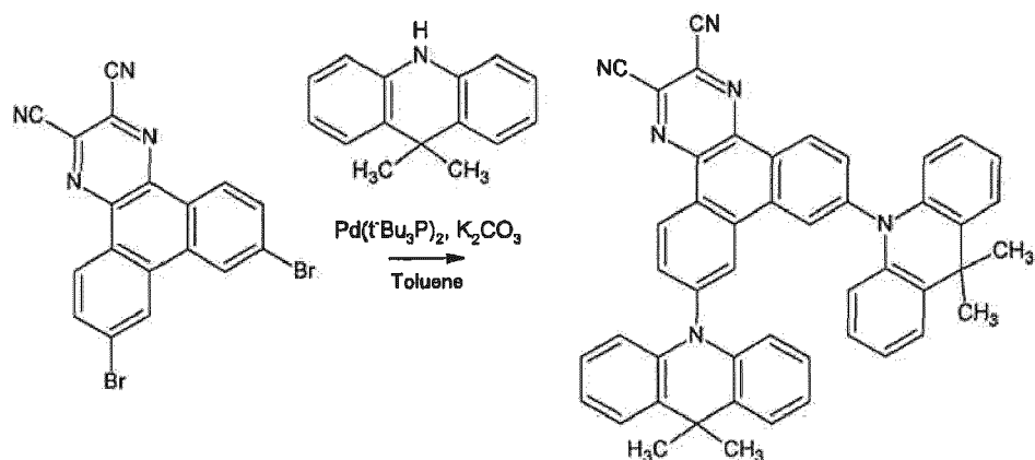
[Chemical formula 63]
