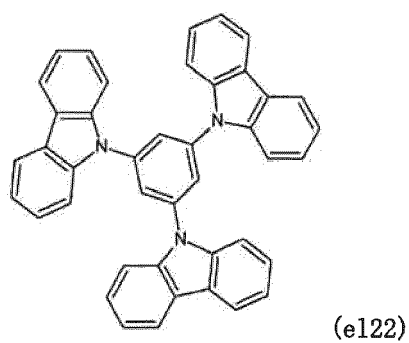
[Chemical formula 141]
