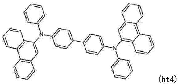
[Chemical formula 80]
