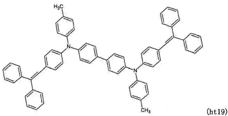
[Chemical formula 95]
