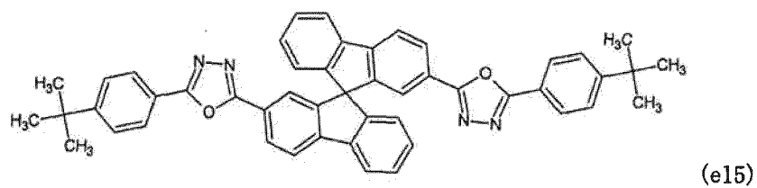
[Chemical formula 124]
