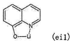
[Chemical formula 201]
