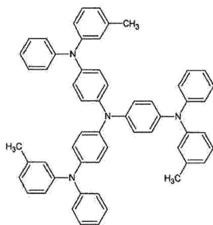
[Chemical formula 90]
