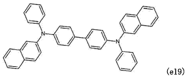
[Chemical formula 128]
