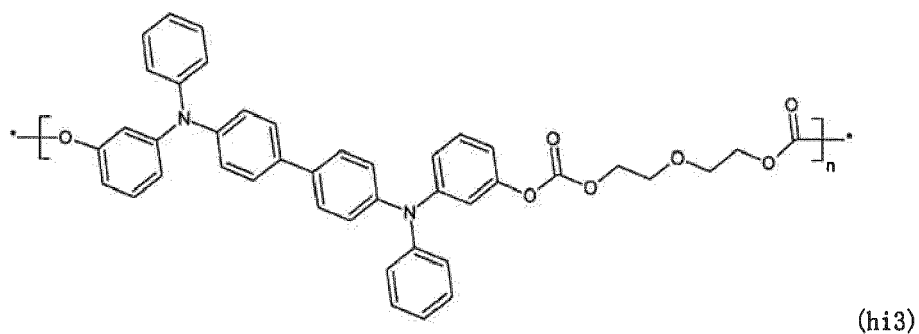
[Chemical formula 71]
