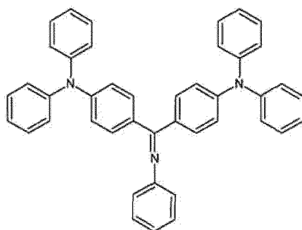
[Chemical formula 109]
