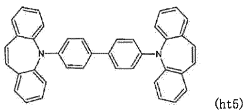
[Chemical formula 81]
