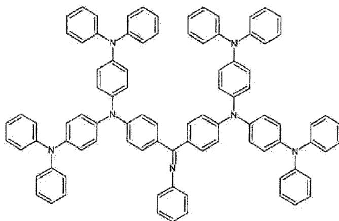
[Chemical formula 110]
