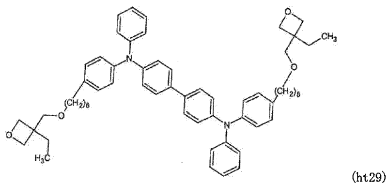
[Chemical formula 104]
