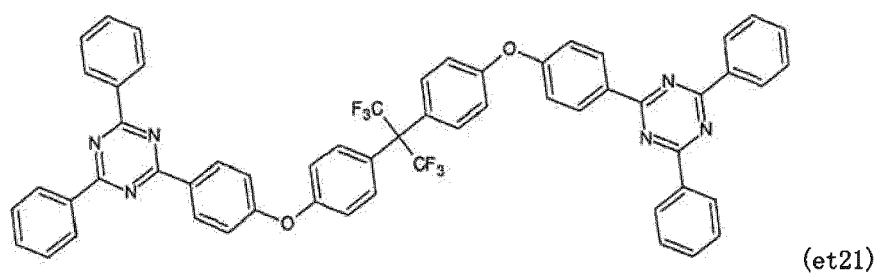
[Chemical formula 191]
