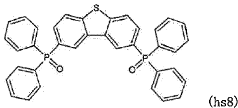
[Chemical formula 167]
