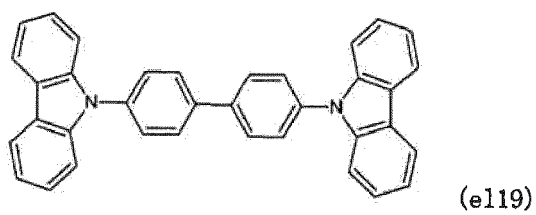
[Chemical formula 138]
