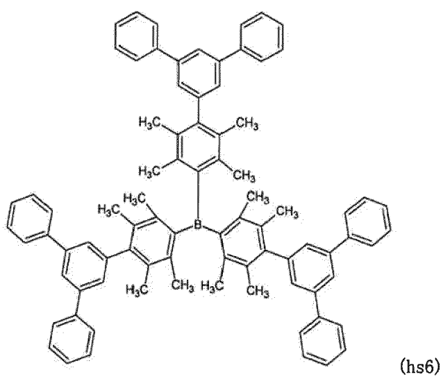
[Chemical formula 165]
