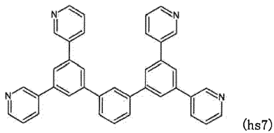
[Chemical formula 165]
