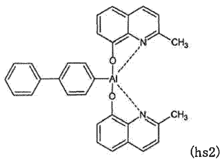
[Chemical formula 161]
