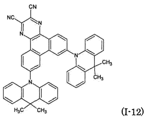
[Chemical formula 45]
