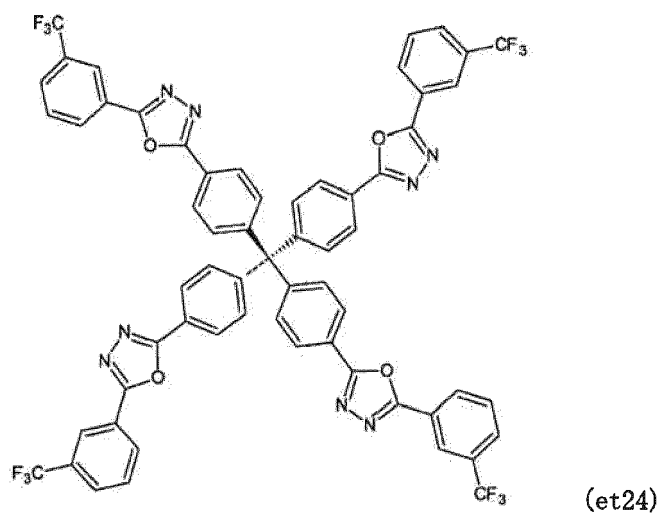
[Chemical formula 194]
