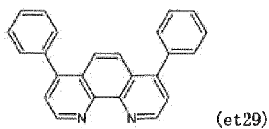
[Chemical formula 199]
