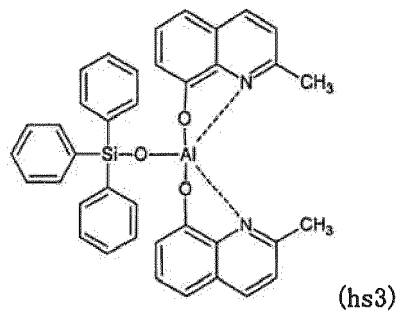
[Chemical formula 162]
