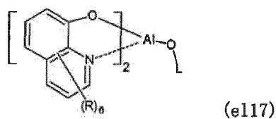
[Chemical formula 136]
