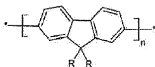
[Chemical formula 154]
