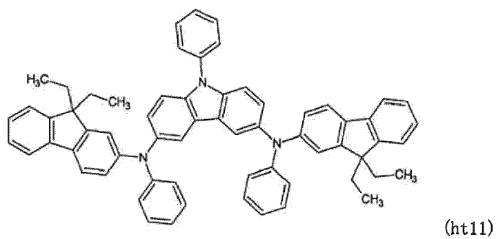
[Chemical formula 87]
