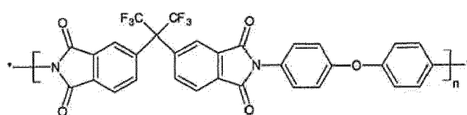
[Chemical formula 100]
