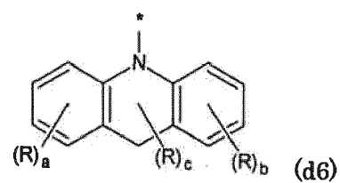
[Chemical formula 21]
