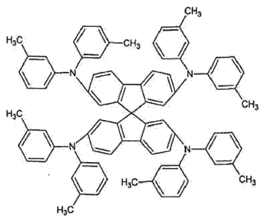
[Chemical formula 98]
