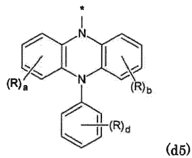
[Chemical formula 20]
