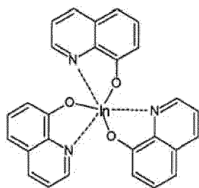
[Chemical formula 175]
