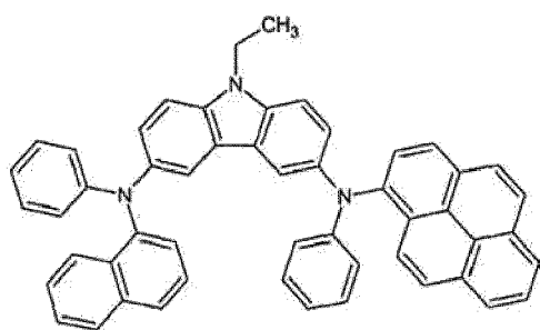
[Chemical formula 89]
