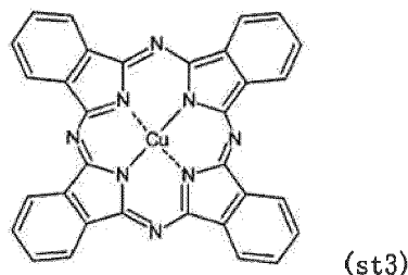
[Chemical formula 207]
