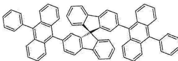
[Chemical formula 153]
