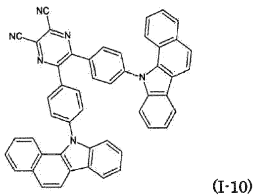
[Chemical formula 44]
