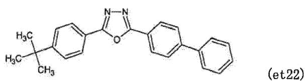
[Chemical formula 192]
