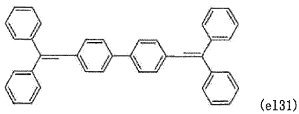
[Chemical formula 150]
