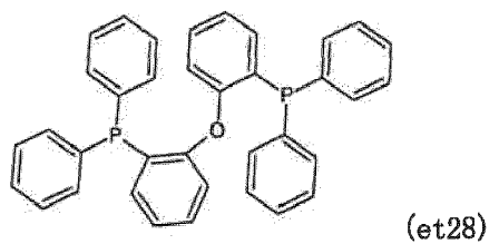
[Chemical formula 198]
