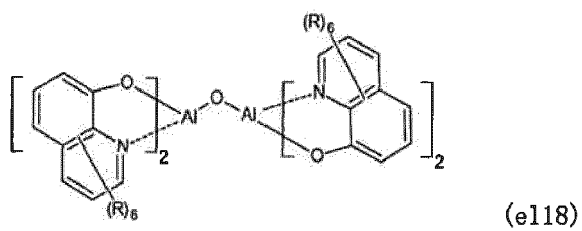
[Chemical formula 137]
