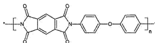
[Chemical formula 100]
