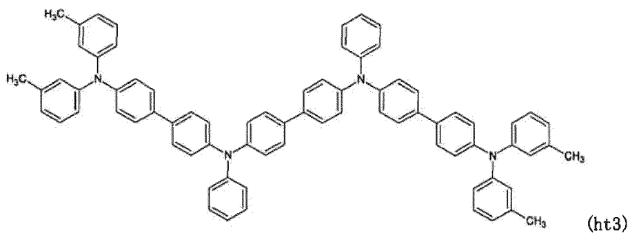
[Chemical formula 78]
