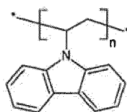
[Chemical formula 155]
