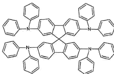
[Chemical formula 122]
