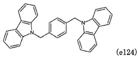
[Chemical formula 143]
