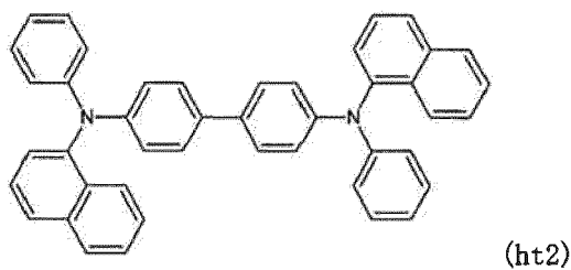
[Chemical formula 77]
