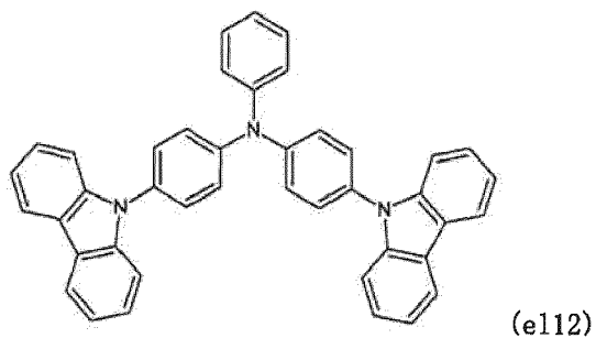
[Chemical formula 131]
