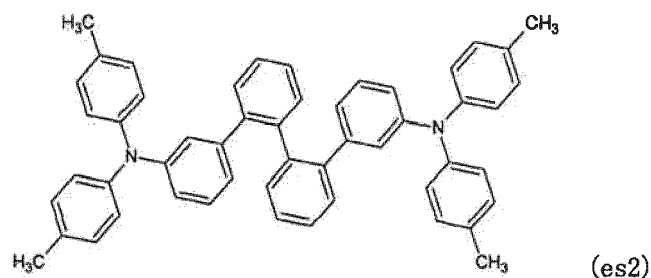
[Chemical formula 116]
