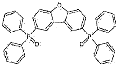
[Chemical formula 213]
