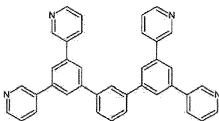
[Chemical formula 220]
