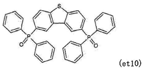
[Chemical formula 180]
