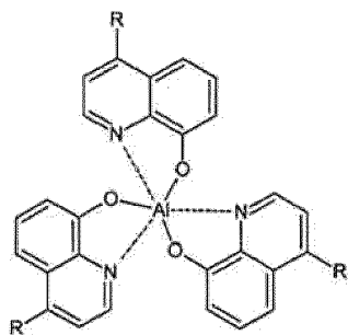
[Chemical formula 176]
