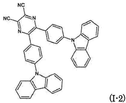
[Chemical formula 36]
