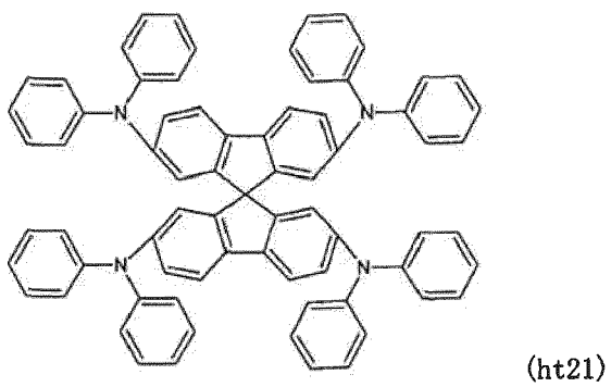
[Chemical formula 96]
