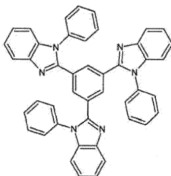
(TPBi)
