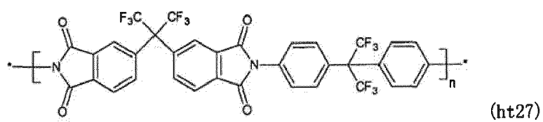
[Chemical formula 103]
