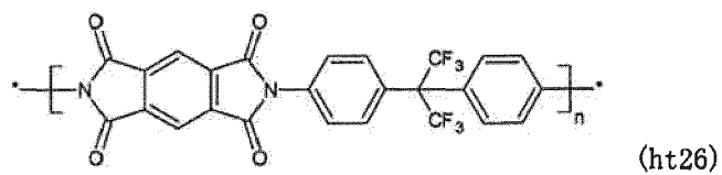
[Chemical formula 102]
