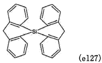
[Chemical formula 146]
