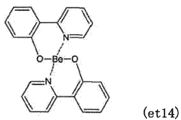
[Chemical formula 184]
