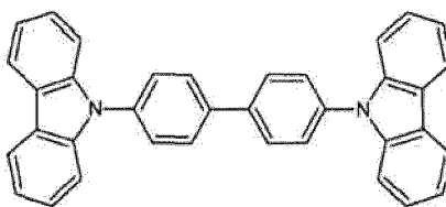
[Chemical formula 218]
