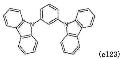
[Chemical formula 142]
