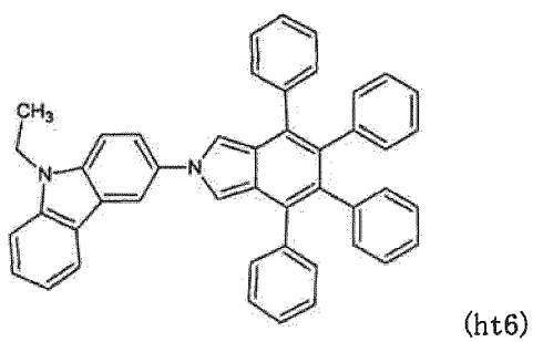
[Chemical formula 81]
