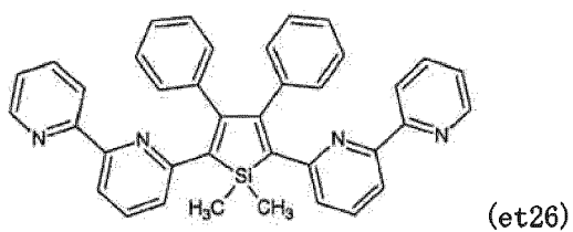
[Chemical formula 196]
