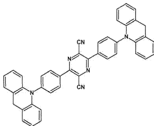
(II-3)
