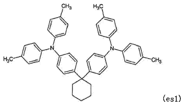
[Chemical formula 115]
