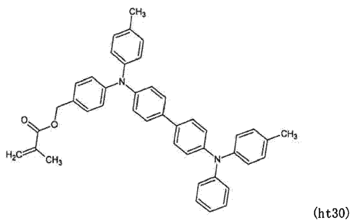
[Chemical formula 106]
