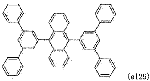
[Chemical formula 148]
