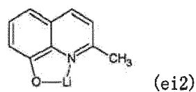
[Chemical formula 201]
