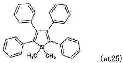
[Chemical formula 195]
