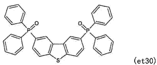
[Chemical formula 199]
