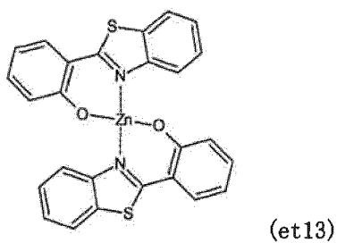
[Chemical formula 183]
