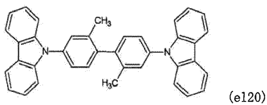
[Chemical formula 138]
