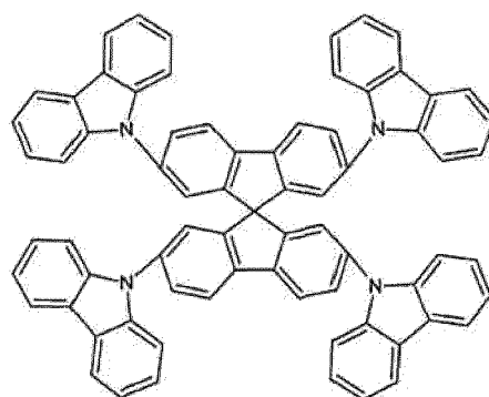
[Chemical formula 99]
