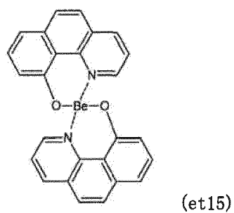
[Chemical formula 185]
