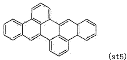
[Chemical formula 208]
