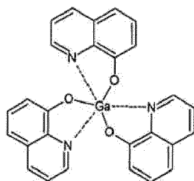
[Chemical formula 174]
