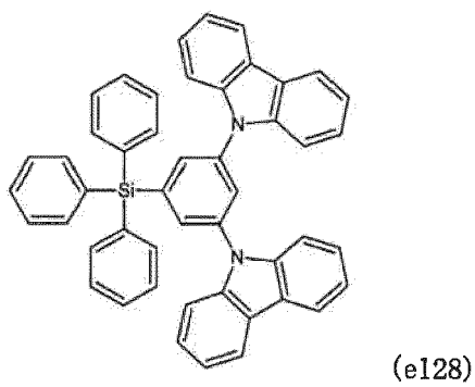
[Chemical formula 146]
