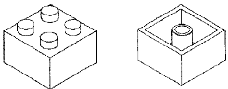
FIG. 8 - PRIOR ART
